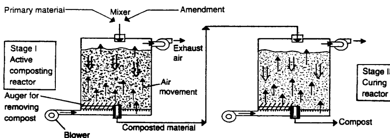
Figure 4-8 Example of a vertical silo composting system
