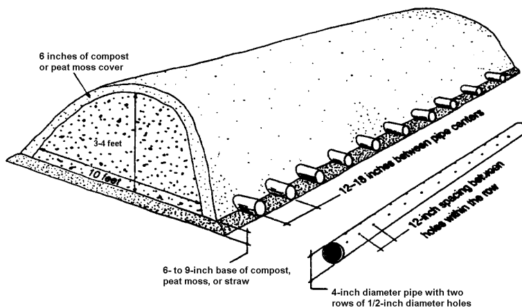
Figure 4-3 Passively aerated windrow method for composting manure.
