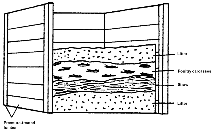
Figure 4-10 Poultry carcass composting bin
