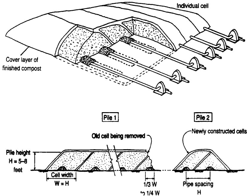
Figure 4-5 Extended aerated static pile layout and dimensions
