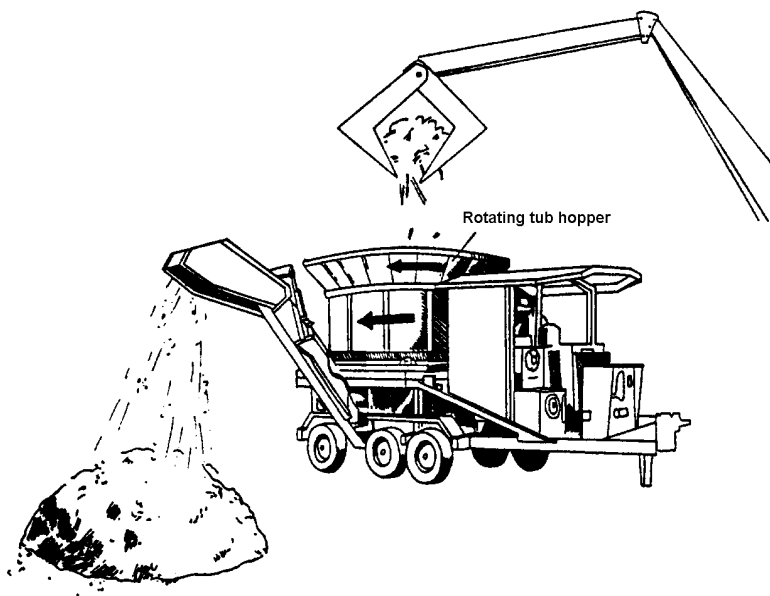
Figure 3-2 Tub Grinder
