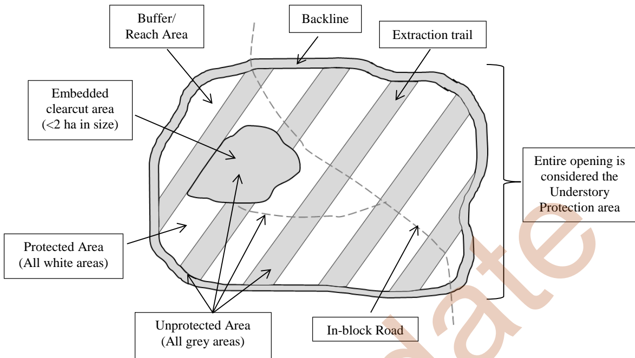
Figure 10-1. Example Understory Protection opening
