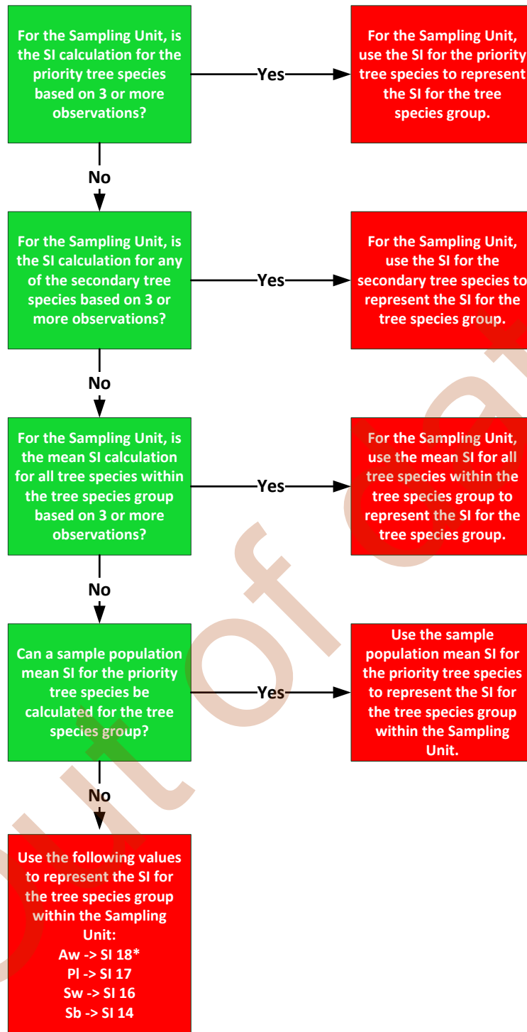
Figure 12-2. Decision key to determine the appropriate SITE_INDEX value to use for a tree species group within a Sampling Unit. Priority tree species are: trembling aspen (Aw) for the Aw tree species group; lodgepole pine (Pl) for the Pl tree species group; white spruce (Sw) for the Sw tree species group; and, black spruce (Sb) for the Sb tree species group.
