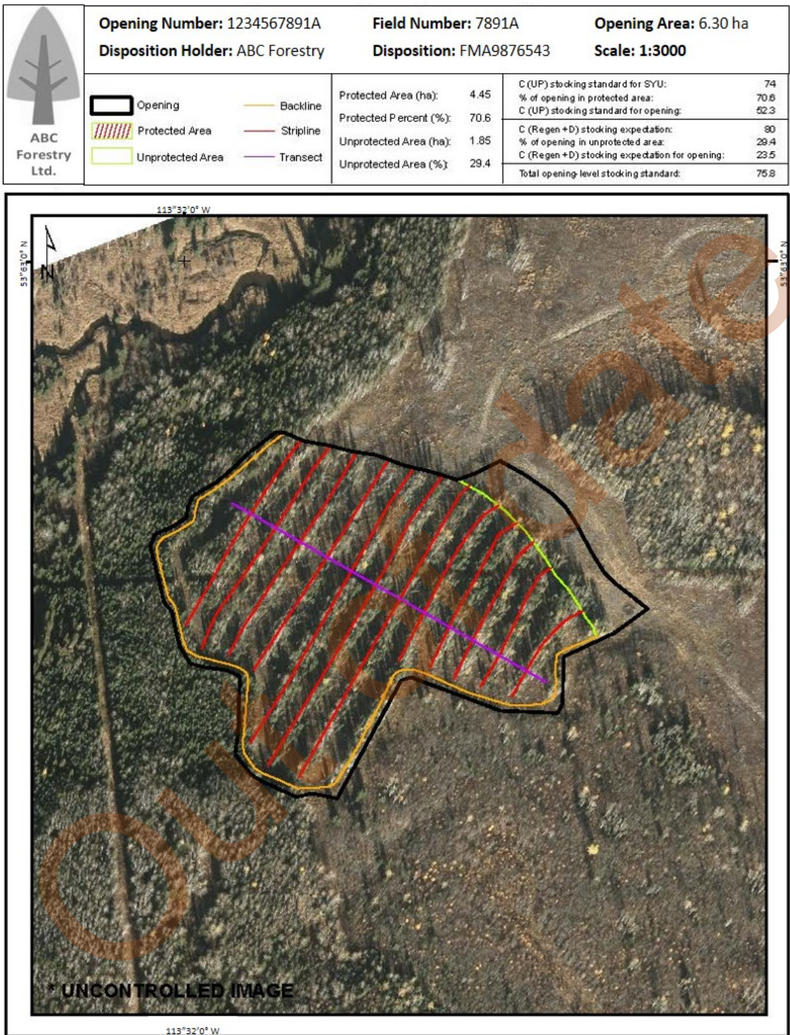
Figure 7-4. Example submission of aerial photo and opening-specific stocking calculations
