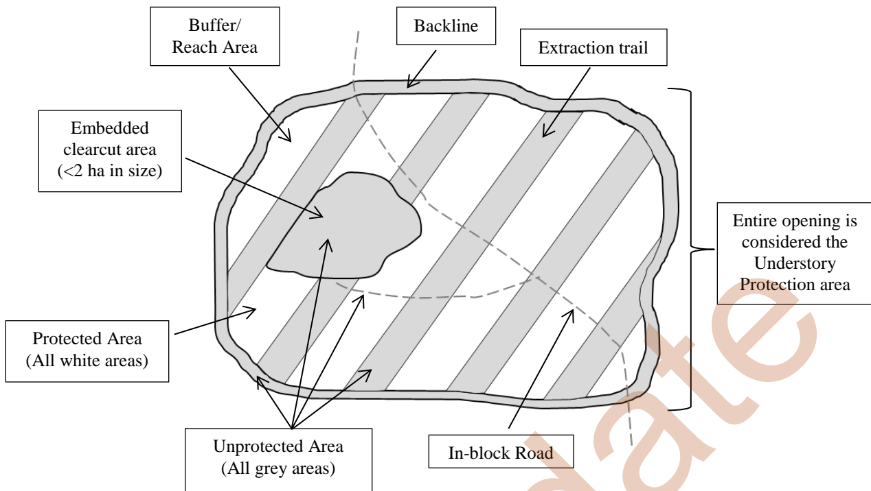
Figure 7-1. Example Understory Protection opening
