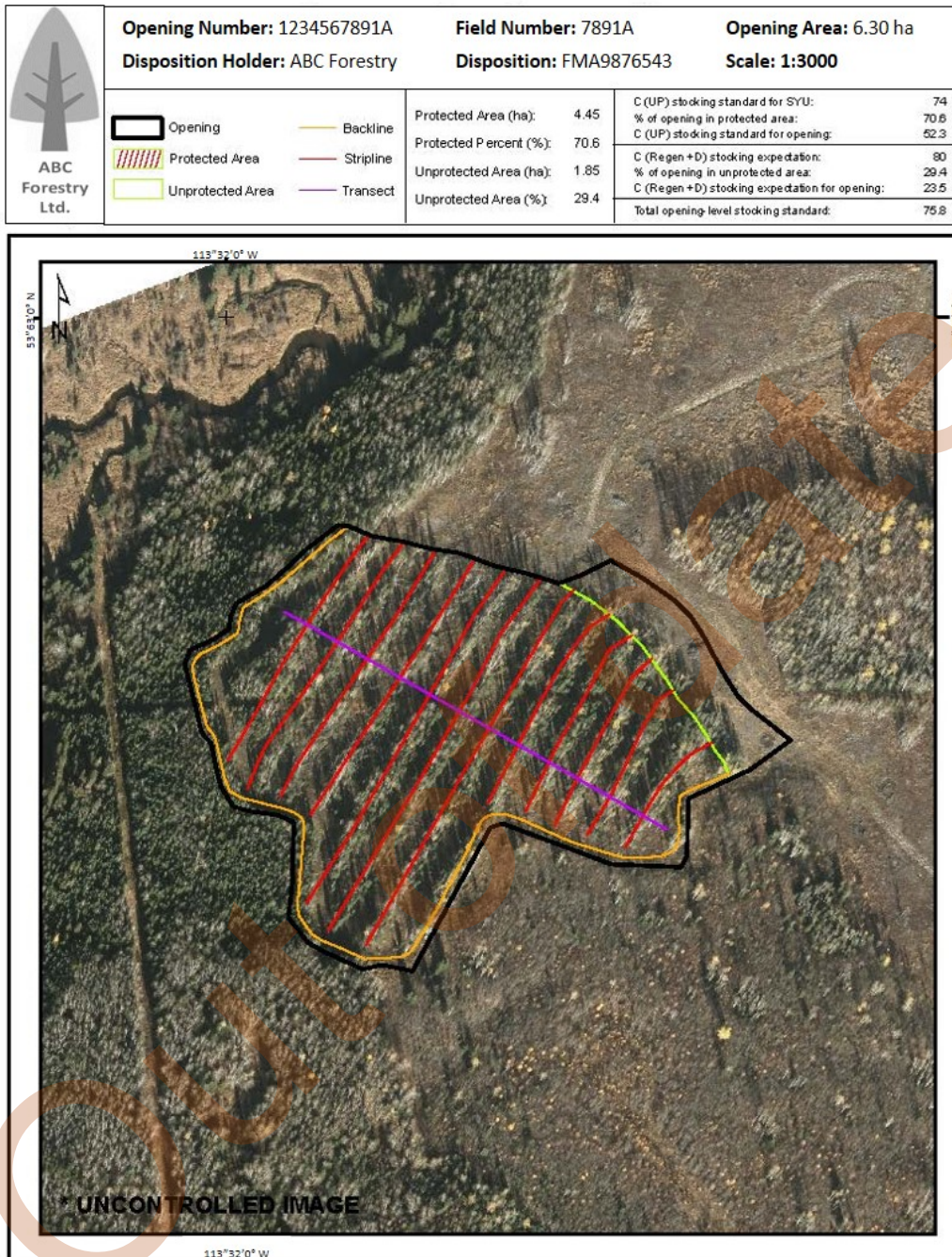
Figure 10-4. Example submission of aerial photo and opening-specific stocking calculations
