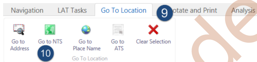
Figure 16 - Address Navigation
