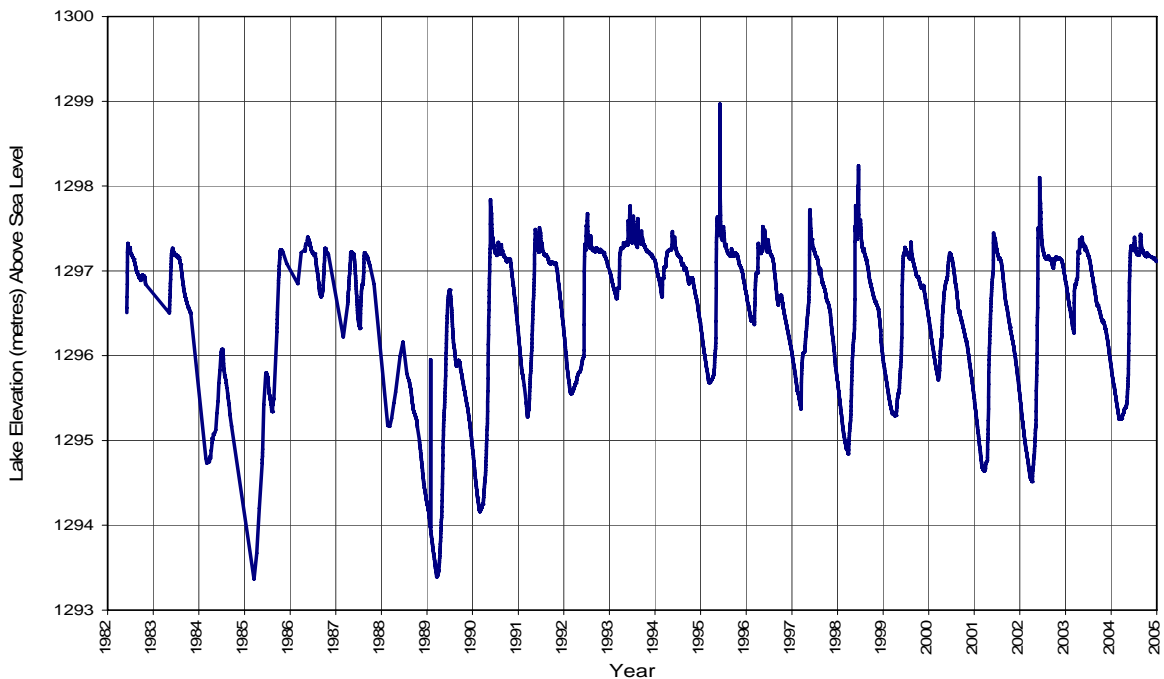
Figure 2. Historic water levels for Chain Lakes Reservoir, Chain Lakes Provincial Park.
