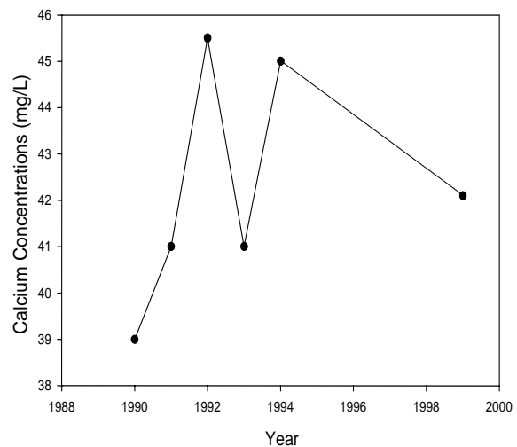
Figure 6b. Calcium concentrations (mg/L) in Chain Lakes Reservoir, south basin, since 1990.
