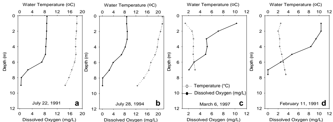
Figure 3. Temperature (dashed line) and DO (solid line) profiles during summer (a, b) and winter (c, d) stratification in north (a, c) and south (b, d) basins of Chain Lakes Reservoir.
