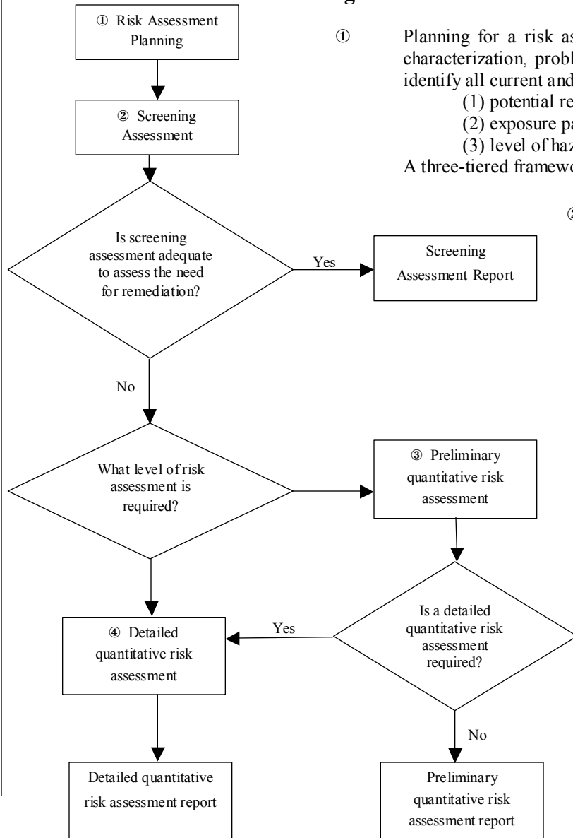
Figure 4.3 Risk Assessment – Decisions on Level of Detail (CCME 1996a)
