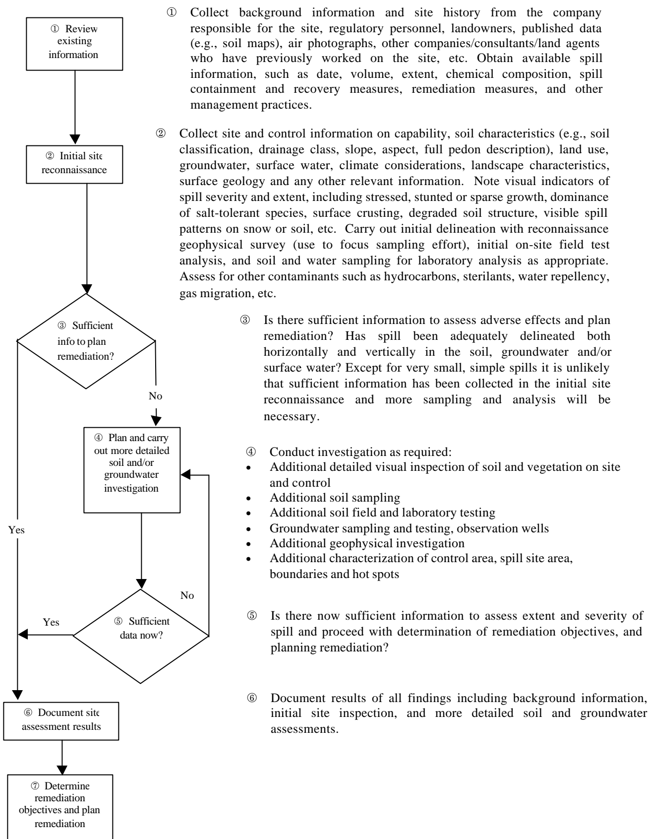
Figure 3.2 Capability Assessment and Site Investigation Flow Chart
