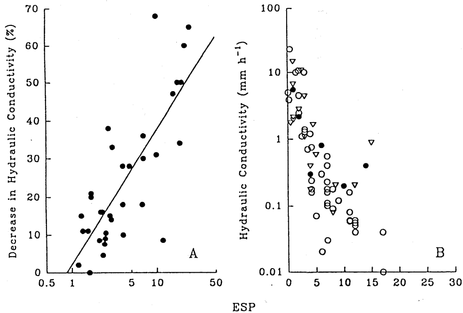
Figure A.4 Reduction in Hydraulic Conductivity Caused by Leaching Soils that have Various Exchangeable Sodium Percentages (ESP) with Tap Water (A-South African Soils, B-Australian Soils, presented in Sumner, 1993)
