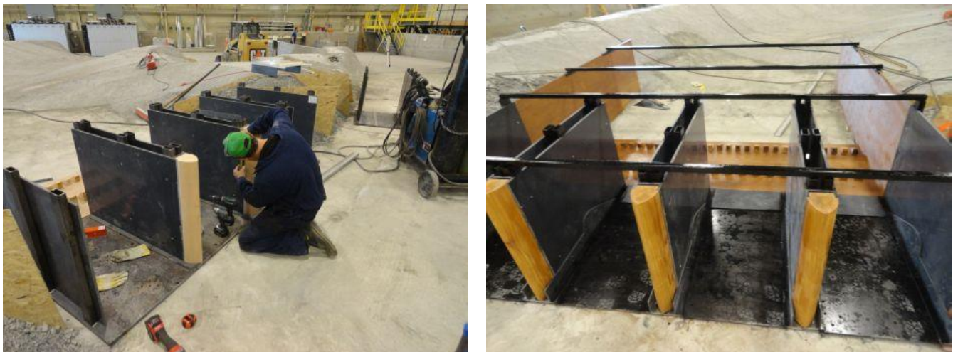
Figure 39. Left: installing the pier noses. Right: installing the support struts, rear retaining walls and rear stilling basin chute blocks.
