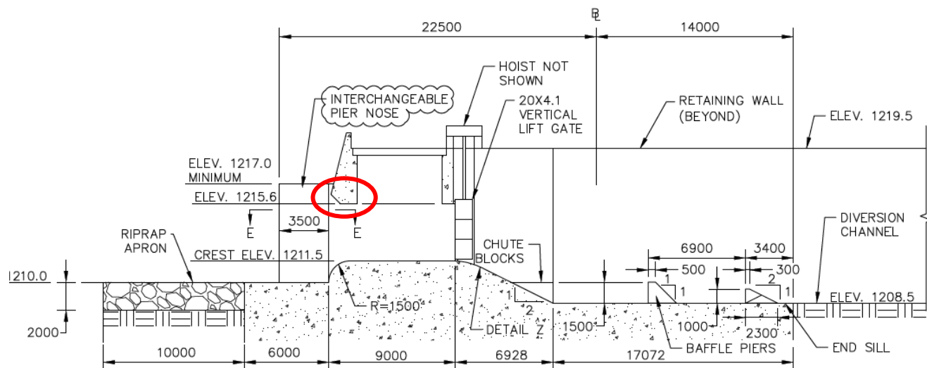
Figure 12. Section view of the diversion inlet structure. Note, the red ellipse highlights the breast wall, which was further modified to a curved profile in the model during the testing.
