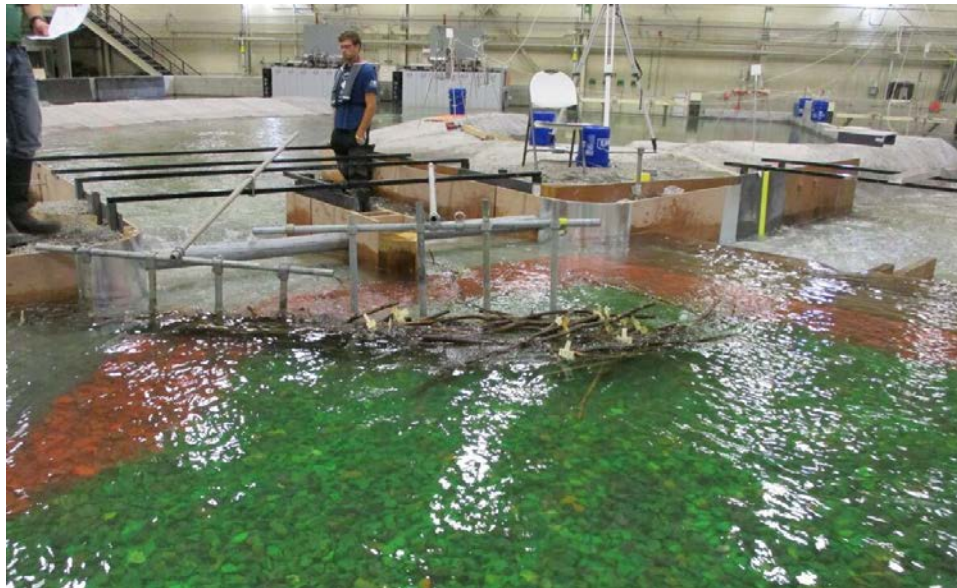
Figure 136. Debris caught on Debris Barrier B.
