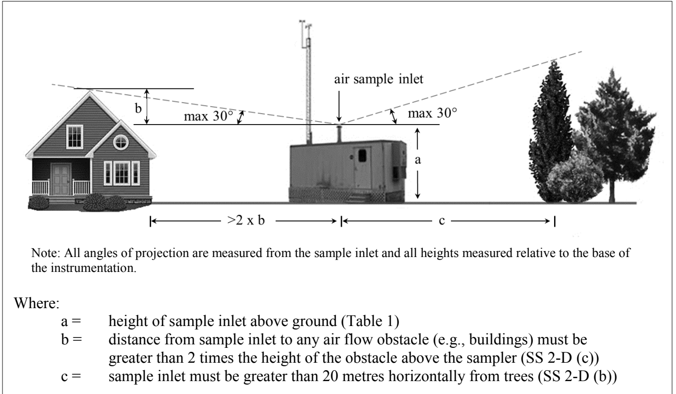
Figure 1 Illustration of distance and height requirements for sampling inlets for a standard continuous ambient air monitoring site
