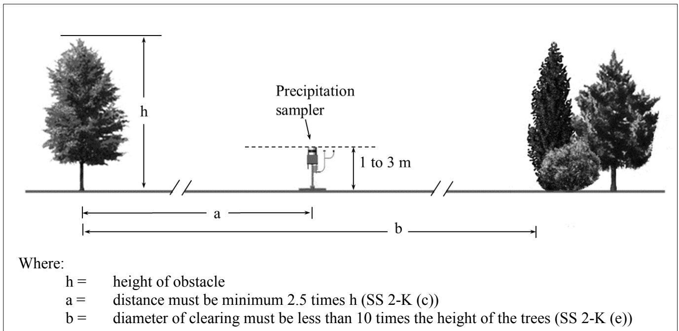
Figure 4 Illustration of precipitation sampler siting
