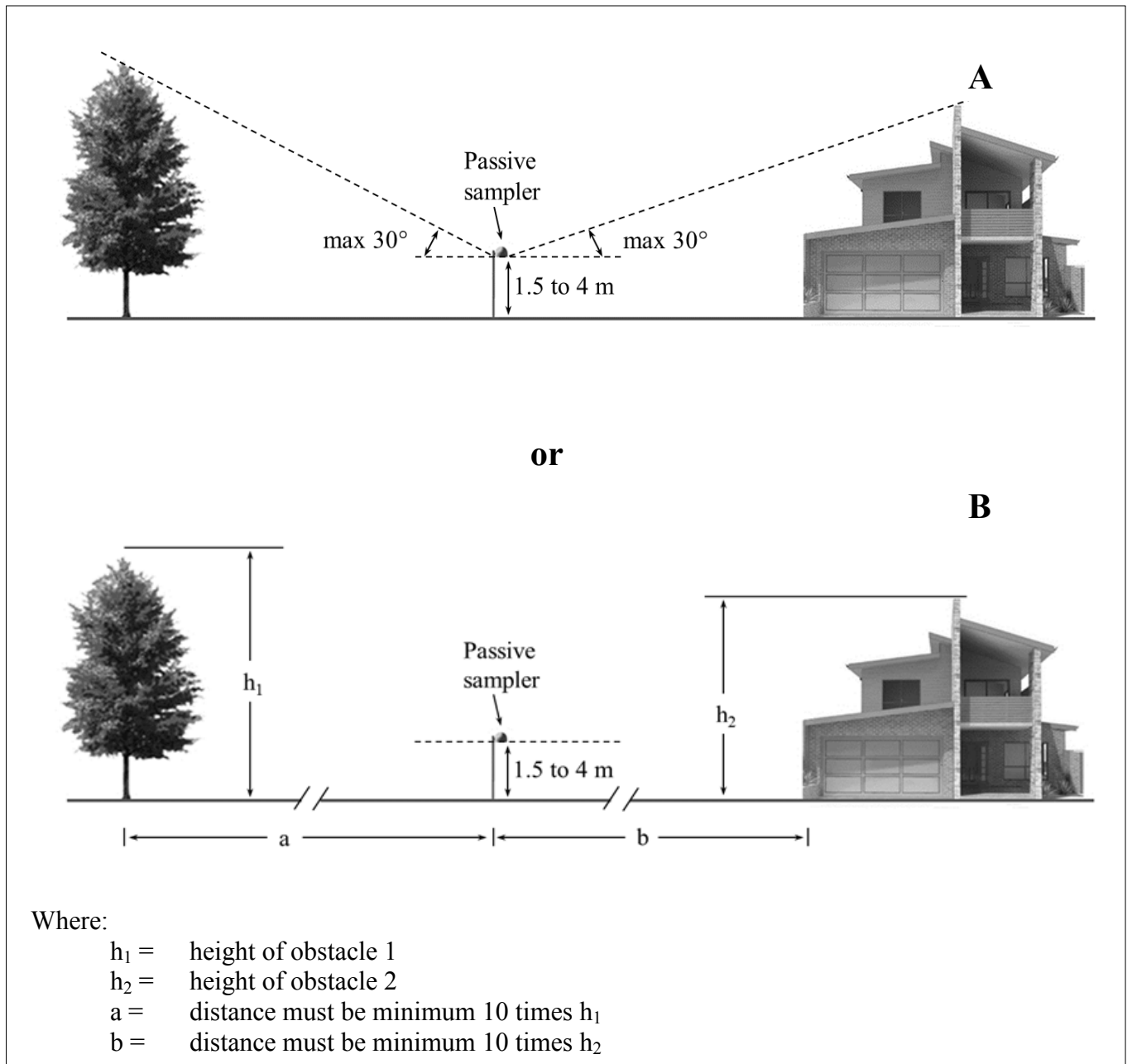
Figure 3 Illustrations of distance and height requirements, A or B, for passive samplers
