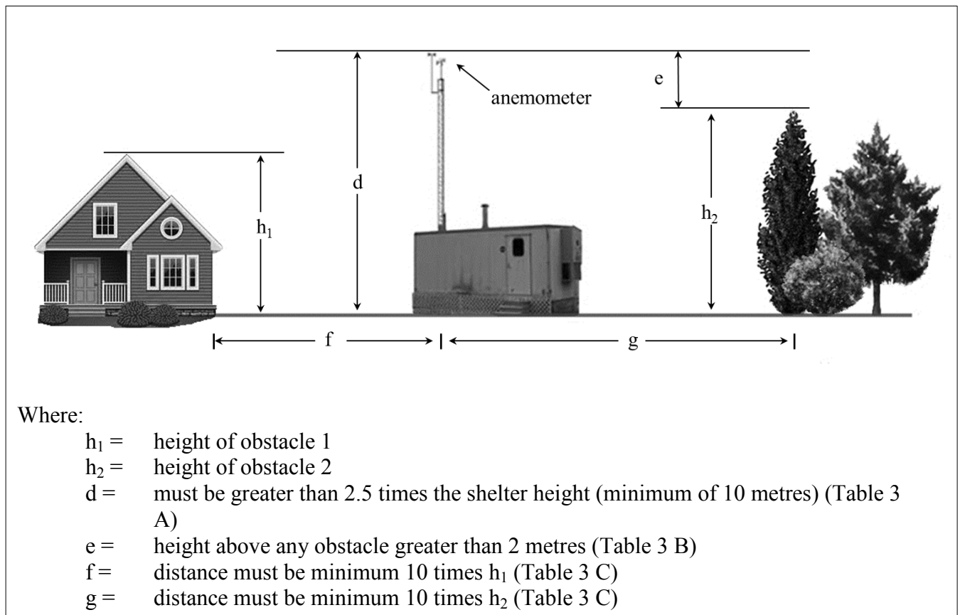
Figure 2 Illustration of distance and height requirements for siting wind instruments
