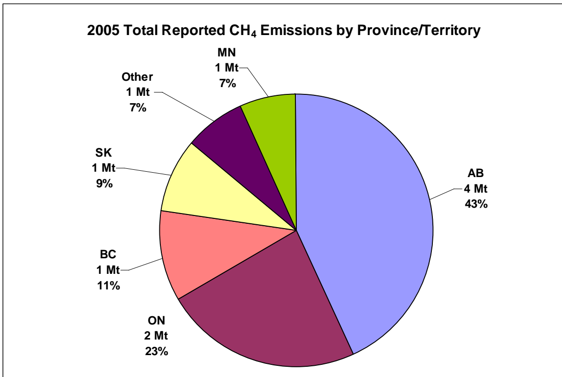
Figure 10: 2005 total reported CH 4 emissions by province/territory.
