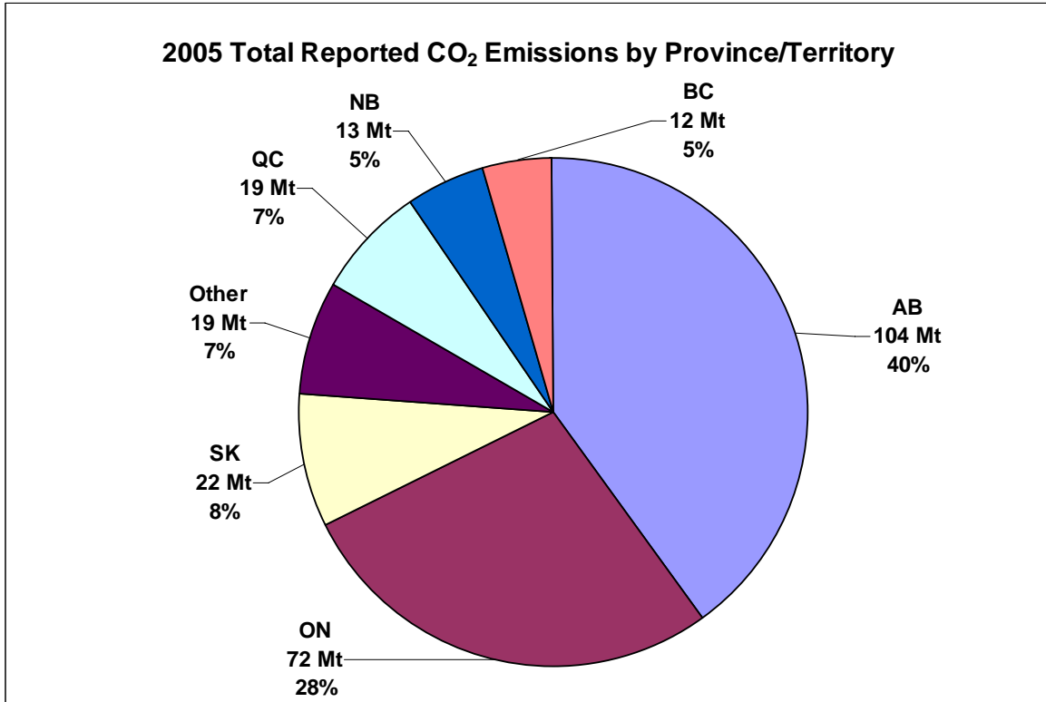
Figure 9: 2005 total reported CO 2 emissions by province/territory.
