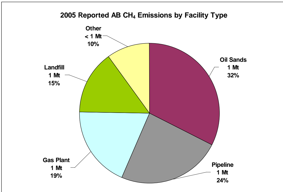
Figure 5: 2005 reported Alberta CH 4 emissions by facility type.
