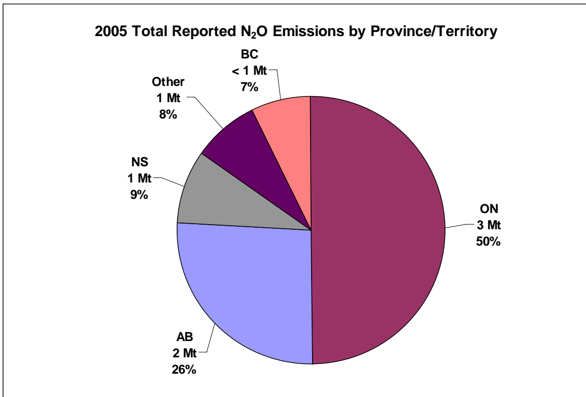
Figure 11: 2005 total reported N 2 O emissions by province/territory.
