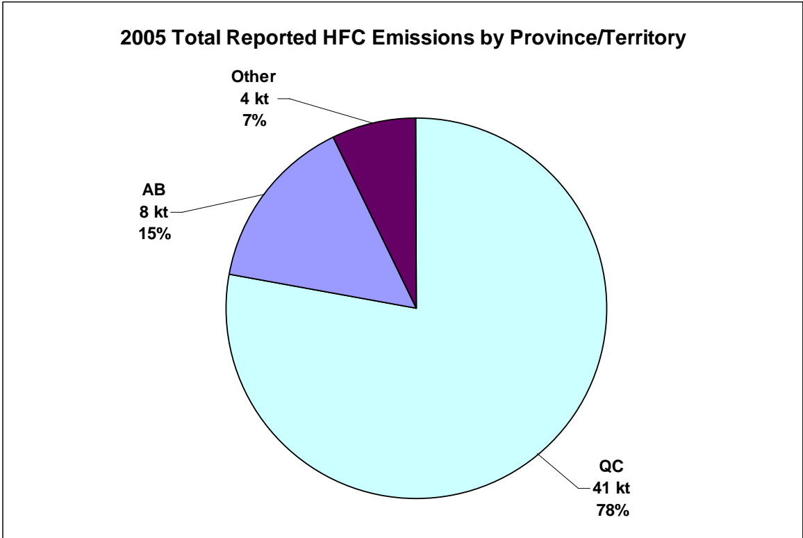
Figure 12: 2005 total reported HFC emissions by province/territory in kt.
