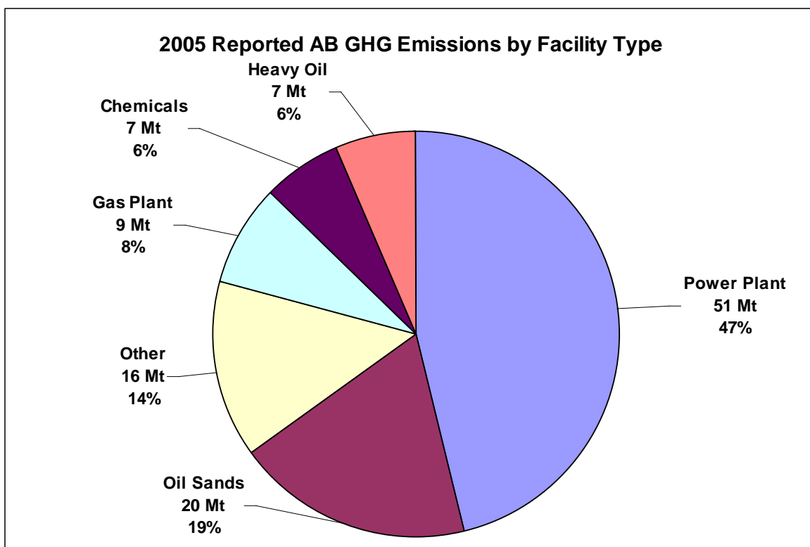
Figure 2: 2005 reported Alberta GHG emissions by facility type.
