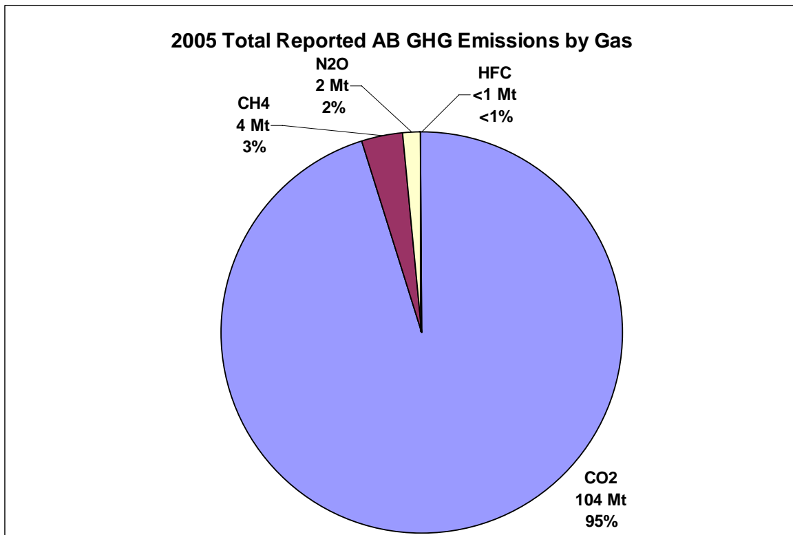
Figure 1: 2005 reported Alberta GHG emissions by gas.
