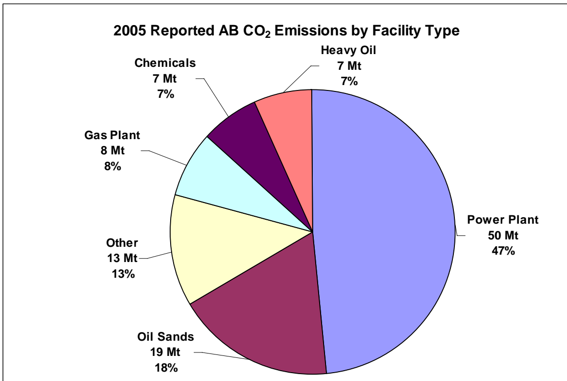
Figure 4: 2005 reported Alberta CO 2 emissions by facility type.
