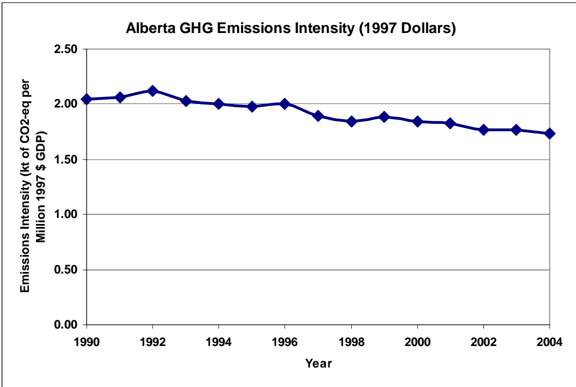
Figure 15: Alberta GHG emissions intensity (1997 Dollars).
