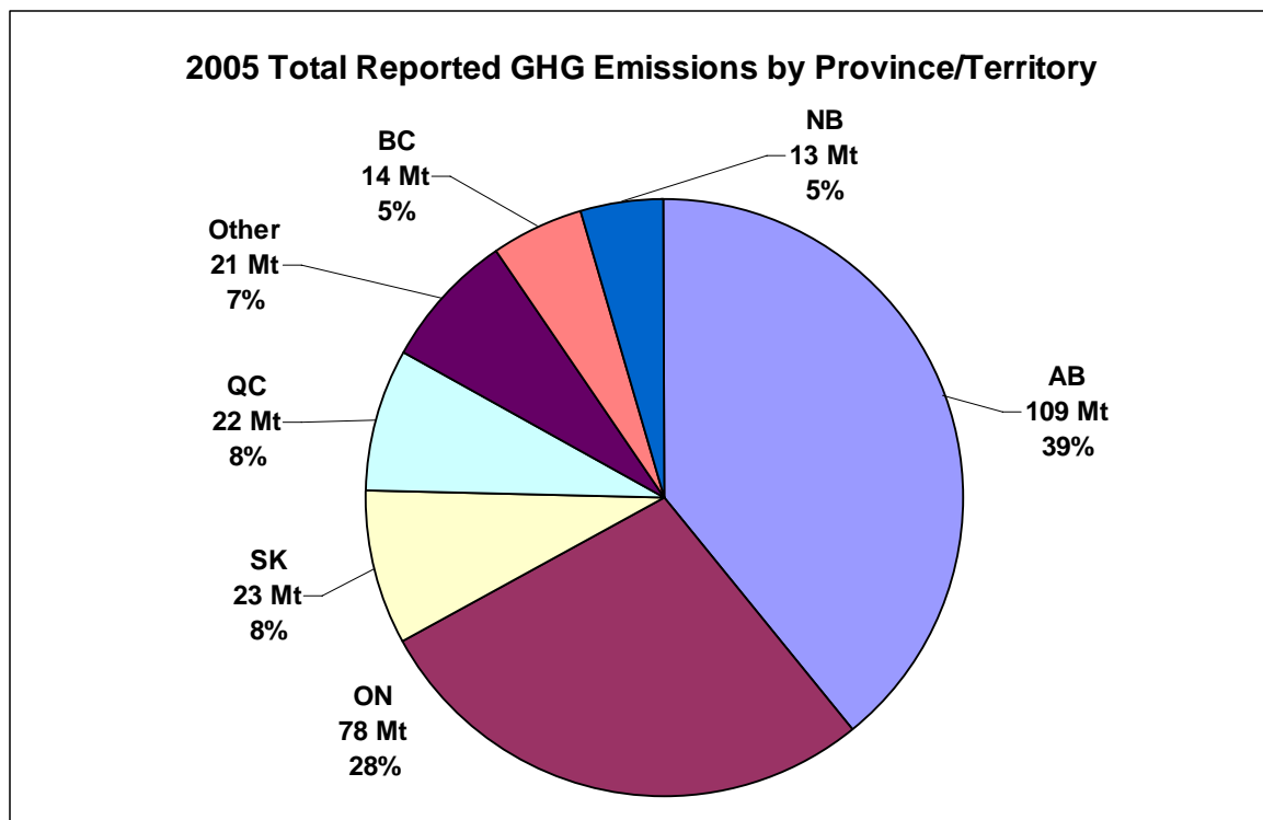
Figure 8: 2005 total reported GHG emissions by province/territory.
