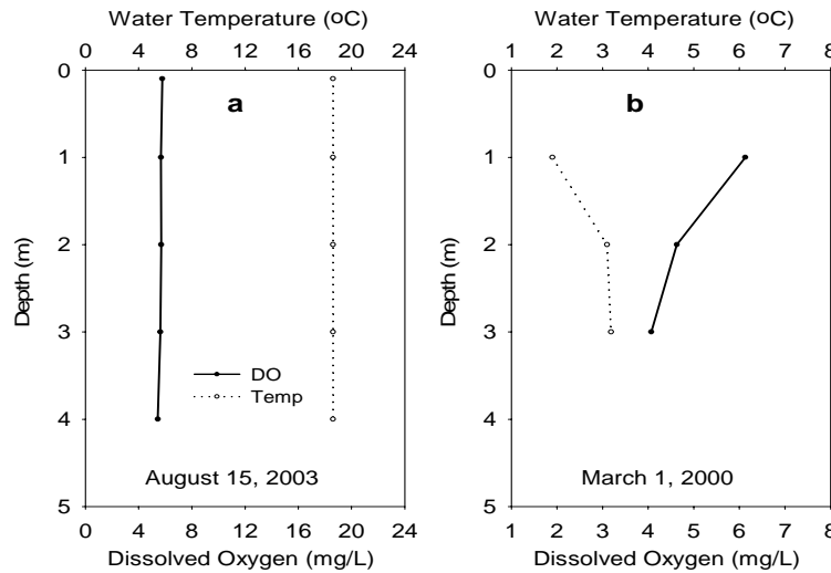
Figure 3. Summer mixing (a) and winter stratification (b) in Winagami Lake.
