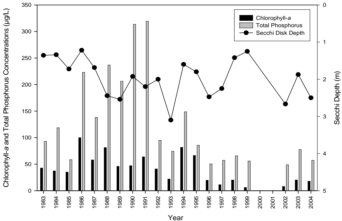
Figure 5. Mean summer (May – October) chlorophyll-a concentrations, total phosphorus concentrations and Secchi depth from 1983-2004.
