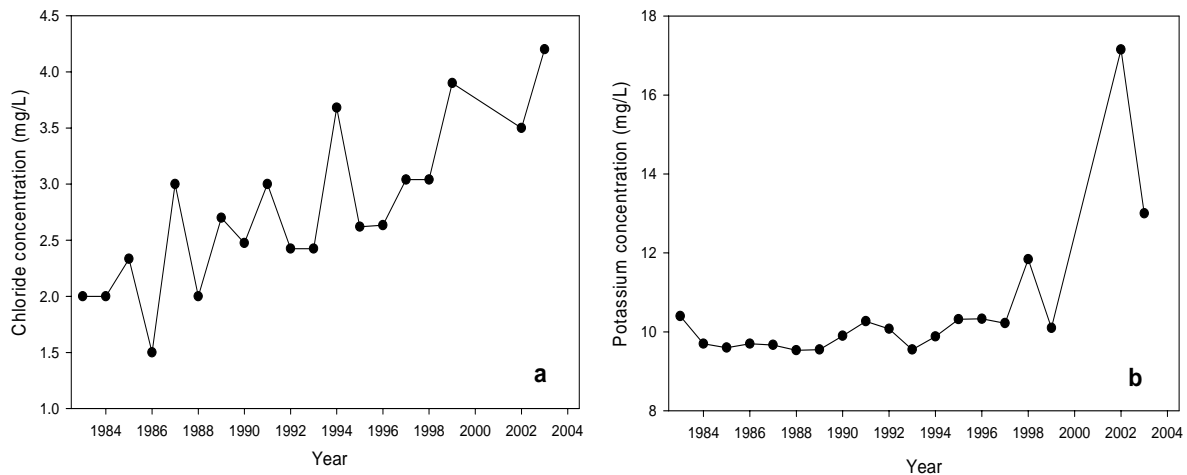
Figure 6. Chloride (a) and potassium (b) concentrations in Winagami Lake from 1983-2004.
