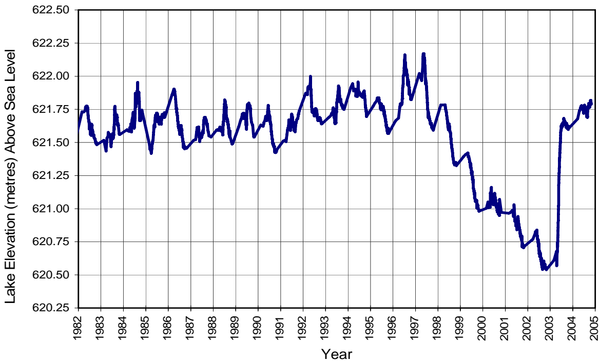
Figure 2. Historic water levels for Winagami Lake, Winagami Lake, Provincial Park.
