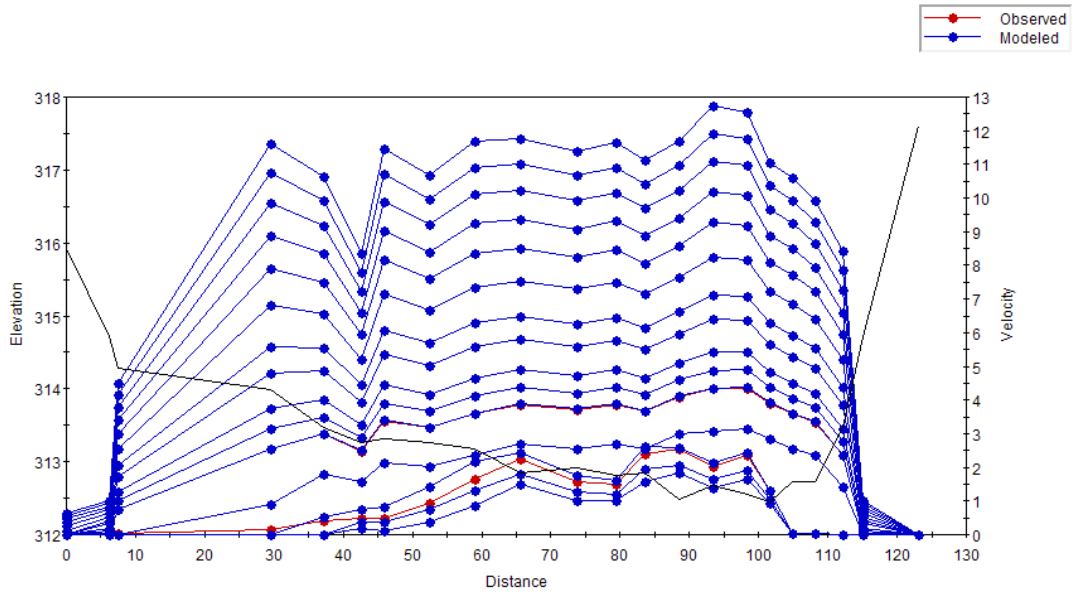
Figure C.11 Plot of the simulated velocity profiles for the Belly River – Study Reach 2 – Cross Section 4.
