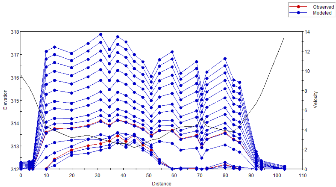
Figure C.14 Plot of the simulated velocity profiles for the Belly River – Study Reach 2 – Cross Section 7.
