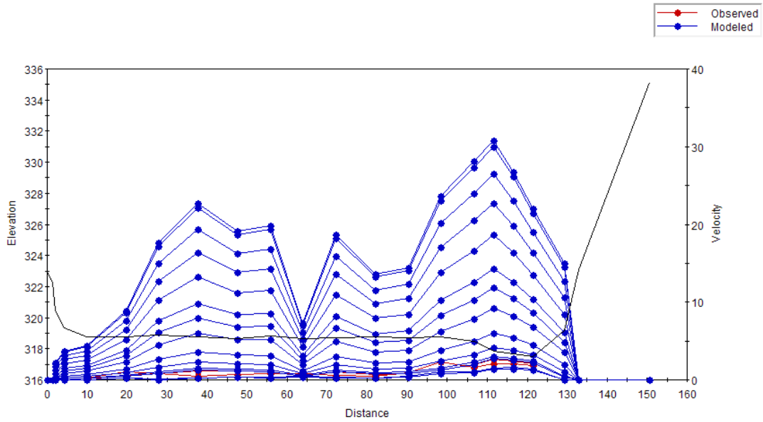
Figure C.17 Plot of the simulated velocity profiles for the Belly River – Study Reach 4 – Cross Section 2.
