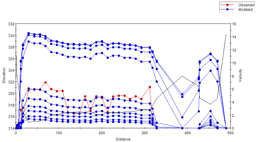
Figure C.35 Plot of the simulated velocity profiles for the Bow River – Study Reach 1 – Cross Section 5.
