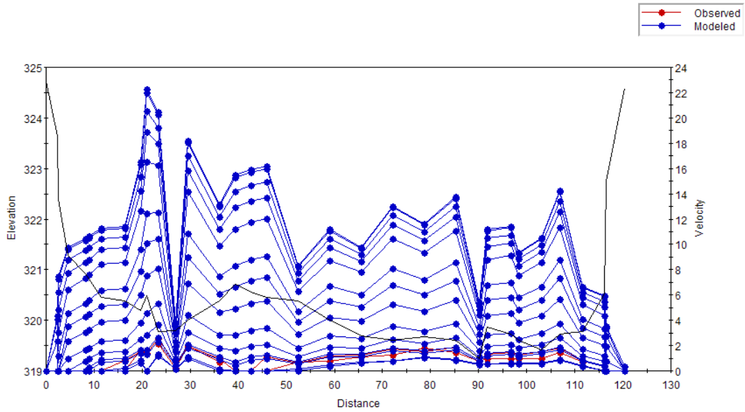
Figure C.19 Plot of the simulated velocity profiles for the Belly River – Study Reach 4 – Cross Section 4.
