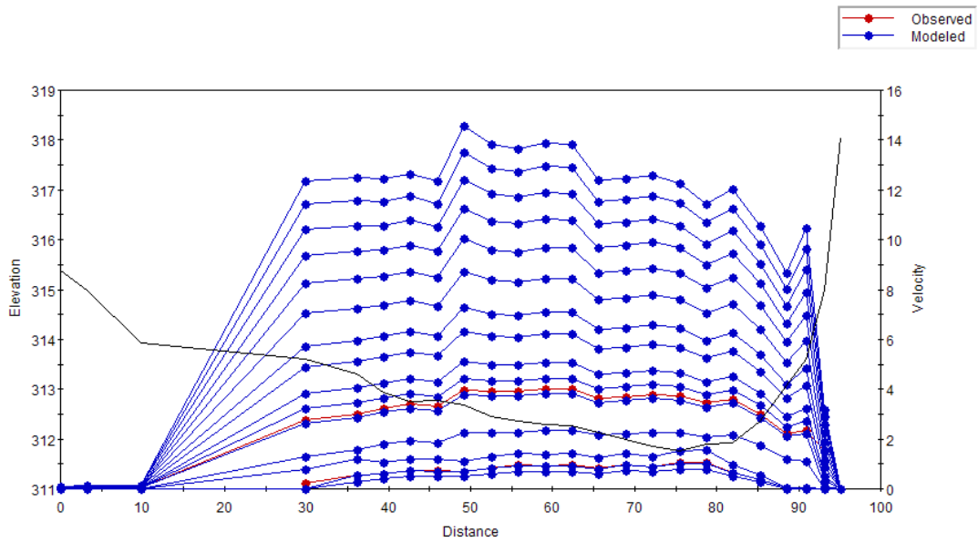
Figure C.12 Plot of the simulated velocity profiles for the Belly River – Study Reach 2 – Cross Section 5.
