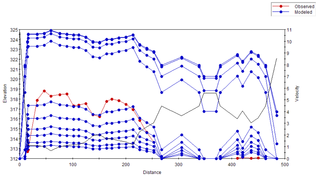
Figure C.34 Plot of the simulated velocity profiles for the Bow River – Study Reach 1 – Cross Section 4.
