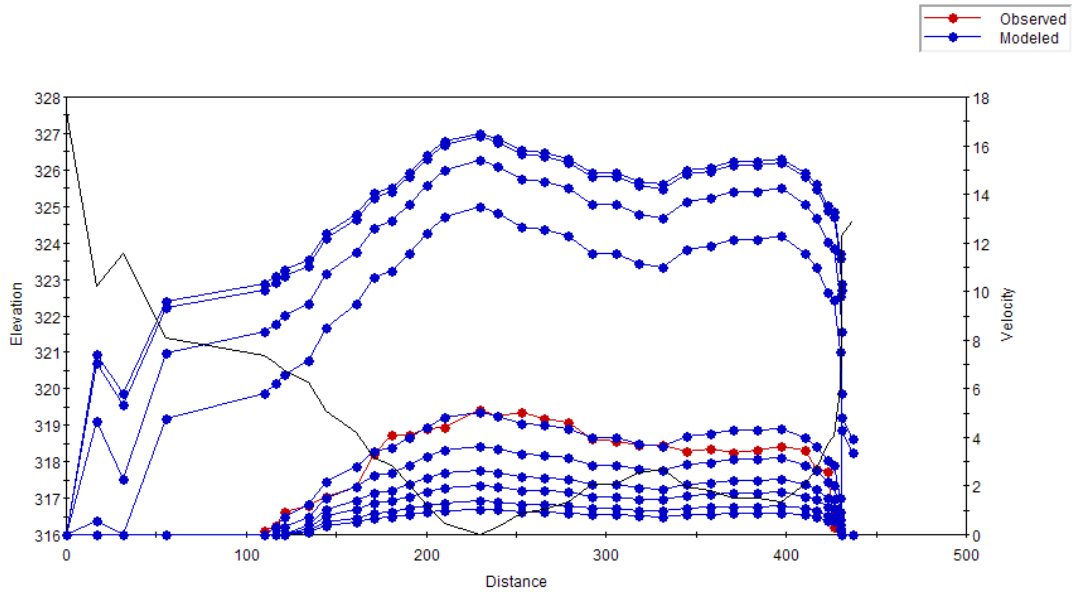
Figure C.37 Plot of the simulated velocity profiles for the Bow River – Study Reach 1 – Cross Section 7.
