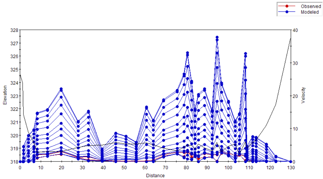
Figure C.18 Plot of the simulated velocity profiles for the Belly River – Study Reach 4 – Cross Section 3.
