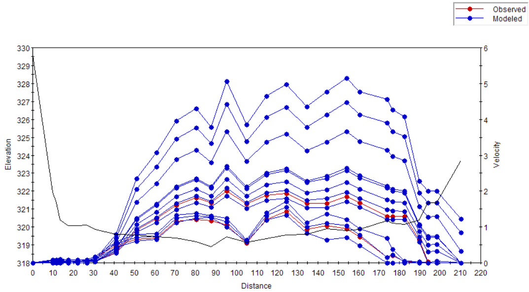
Figure C.5 Plot of the simulated velocity profiles for the Belly River – Study Reach 1 – Cross Section 5.
