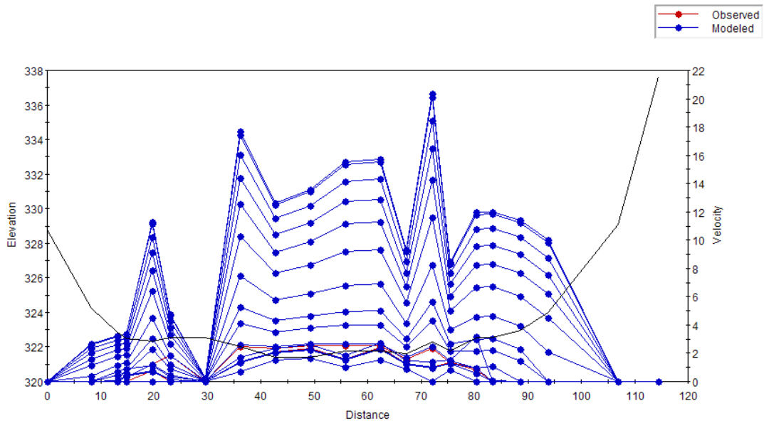
Figure C.24 Plot of the simulated velocity profiles for the Belly River – Study Reach 5 – Cross Section 2.
