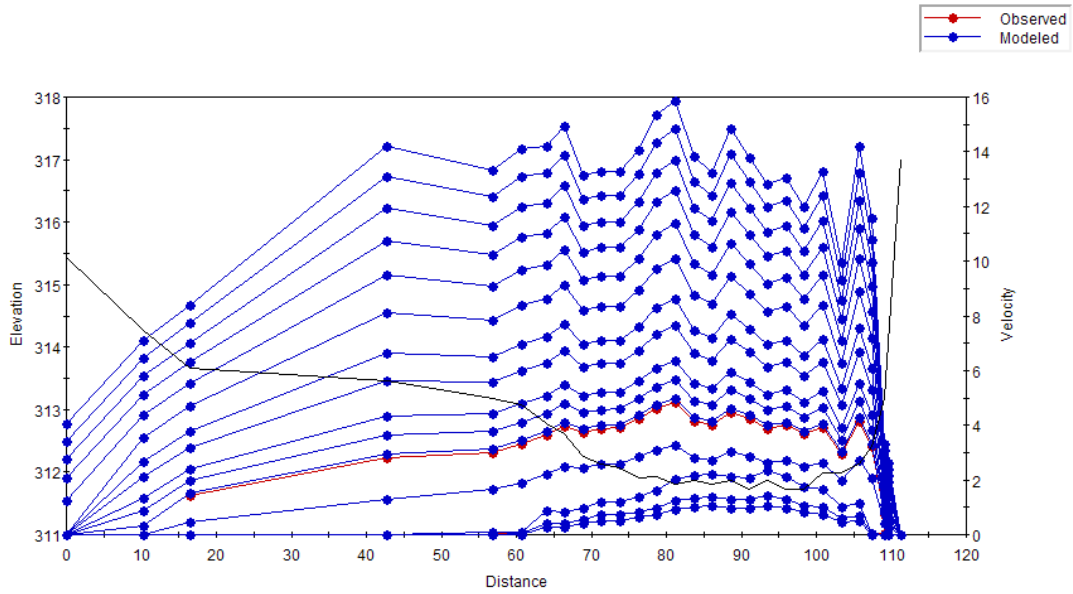
Figure C.9 Plot of the simulated velocity profiles for the Belly River – Study Reach 2 – Cross Section 2.
