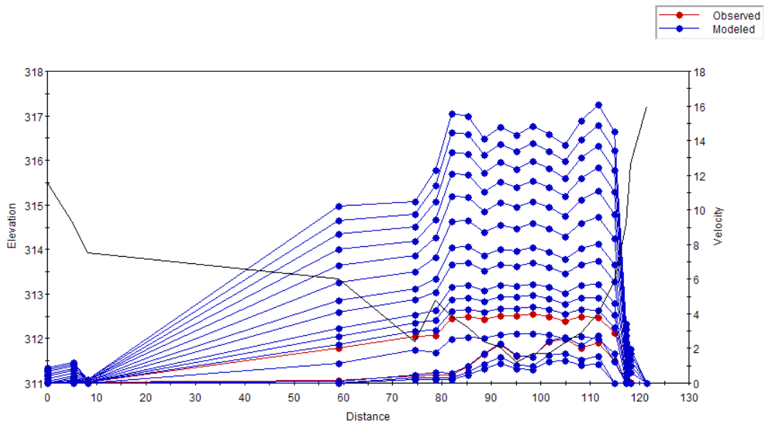
Figure C.10 Plot of the simulated velocity profiles for the Belly River – Study Reach 2 – Cross Section 3.
