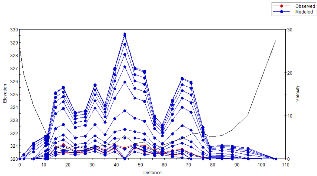
Figure C.23 Plot of the simulated velocity profiles for the Belly River – Study Reach 5 – Cross Section 1.
