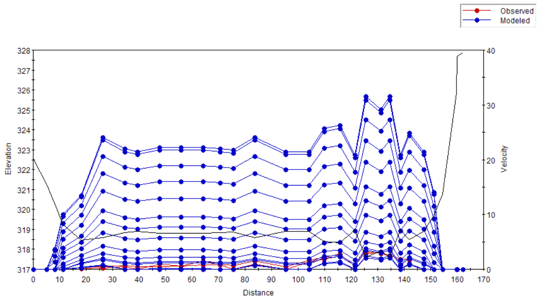
Figure C.16 Plot of the simulated velocity profiles for the Belly River – Study Reach 4 – Cross Section 1.
