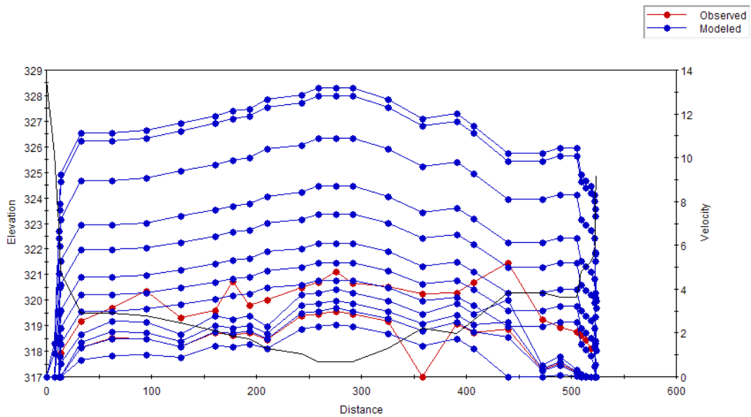
Figure C.38 Plot of the simulated velocity profiles for the Bow River – Study Reach 2 – Cross Section 1.
