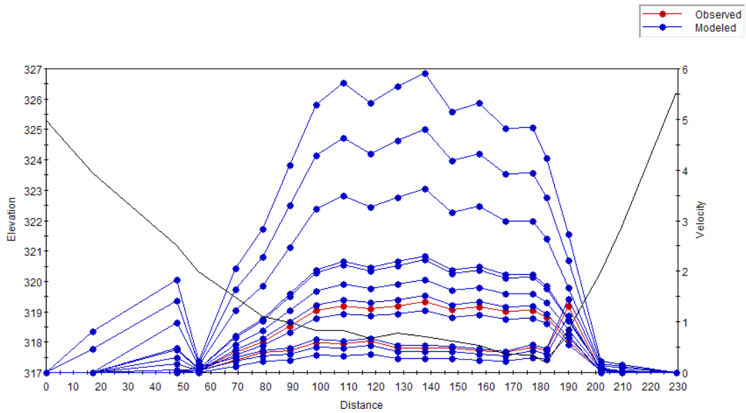
Figure C.3 Plot of the simulated velocity profiles for the Belly River – Study Reach 1 – Cross Section 3.
