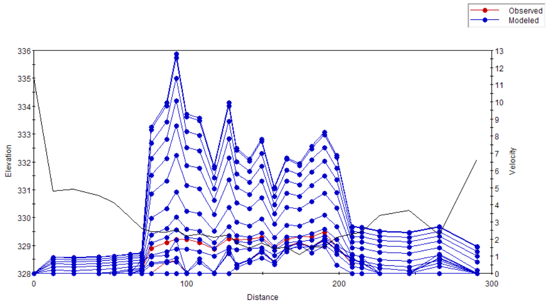
Figure C.30 Plot of the simulated velocity profiles for the Belly River – Study Reach 5 – Cross Section 8.
