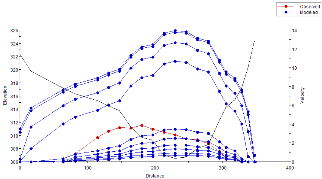
Figure C.32 Plot of the simulated velocity profiles for the Bow River – Study Reach 1 – Cross Section 2.
