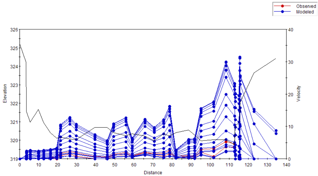
Figure C.20 Plot of the simulated velocity profiles for the Belly River – Study Reach 4 – Cross Section 5.
