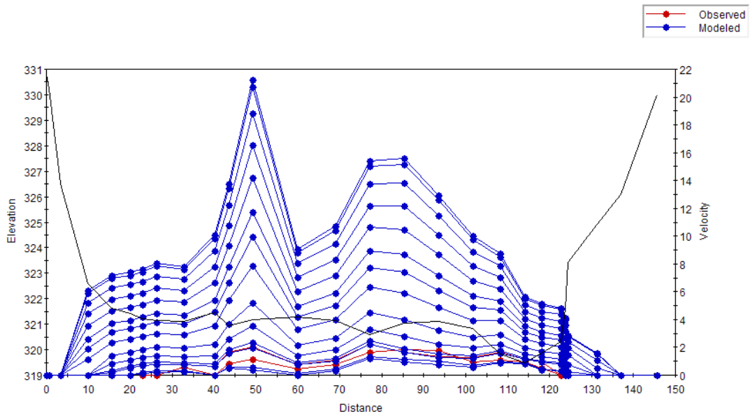
Figure C.21 Plot of the simulated velocity profiles for the Belly River – Study Reach 4 – Cross Section 6.
