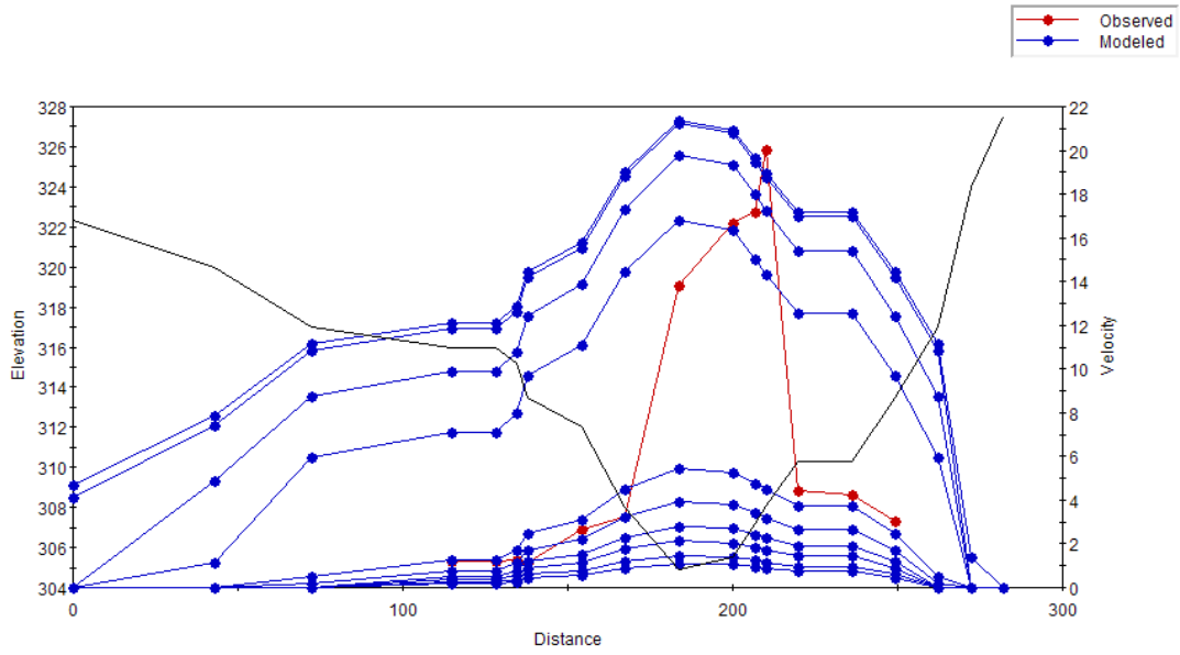
Figure C.31 Plot of the simulated velocity profiles for the Bow River – Study Reach 1 – Cross Section 1.
