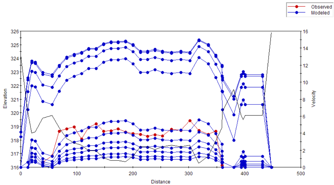
Figure C.36 Plot of the simulated velocity profiles for the Bow River – Study Reach 1 – Cross Section 6.
