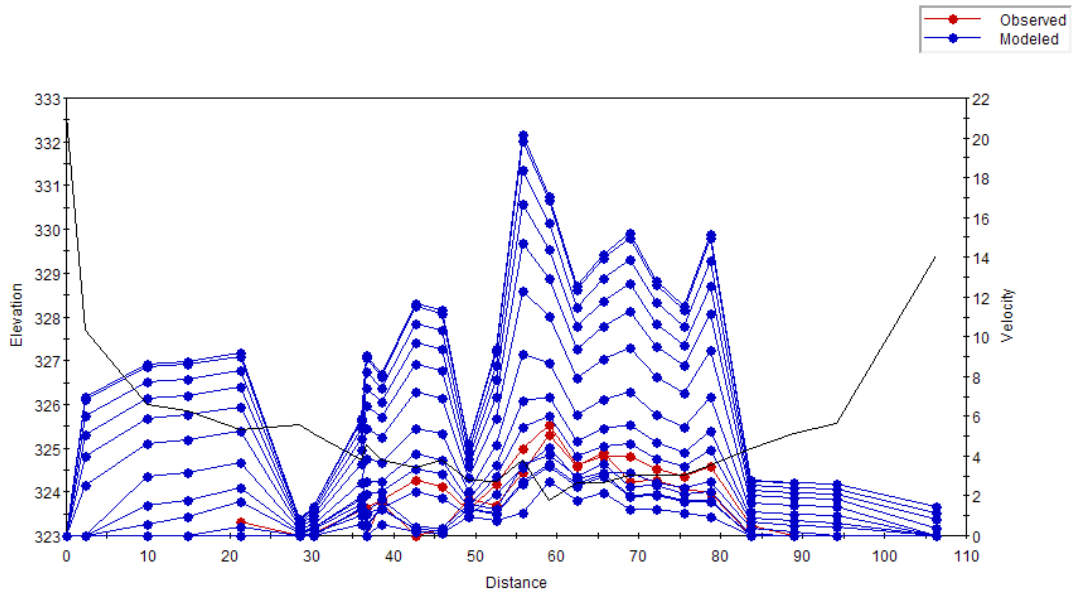
Figure C.29 Plot of the simulated velocity profiles for the Belly River – Study Reach 5 – Cross Section 7.
