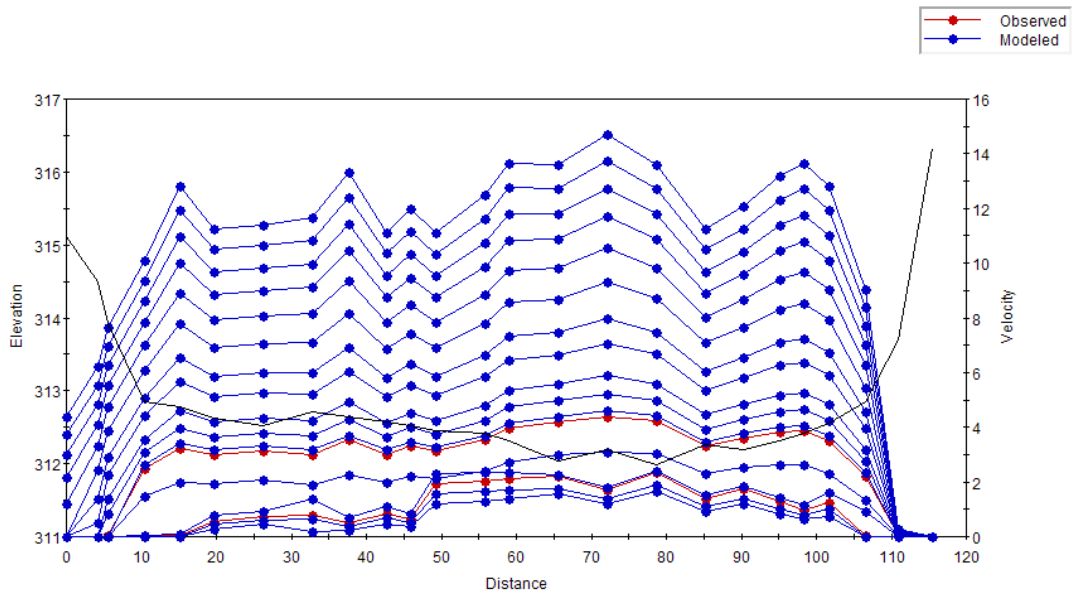
Figure C.8 Plot of the simulated velocity profiles for the Belly River – Study Reach 2 – Cross Section 1.
