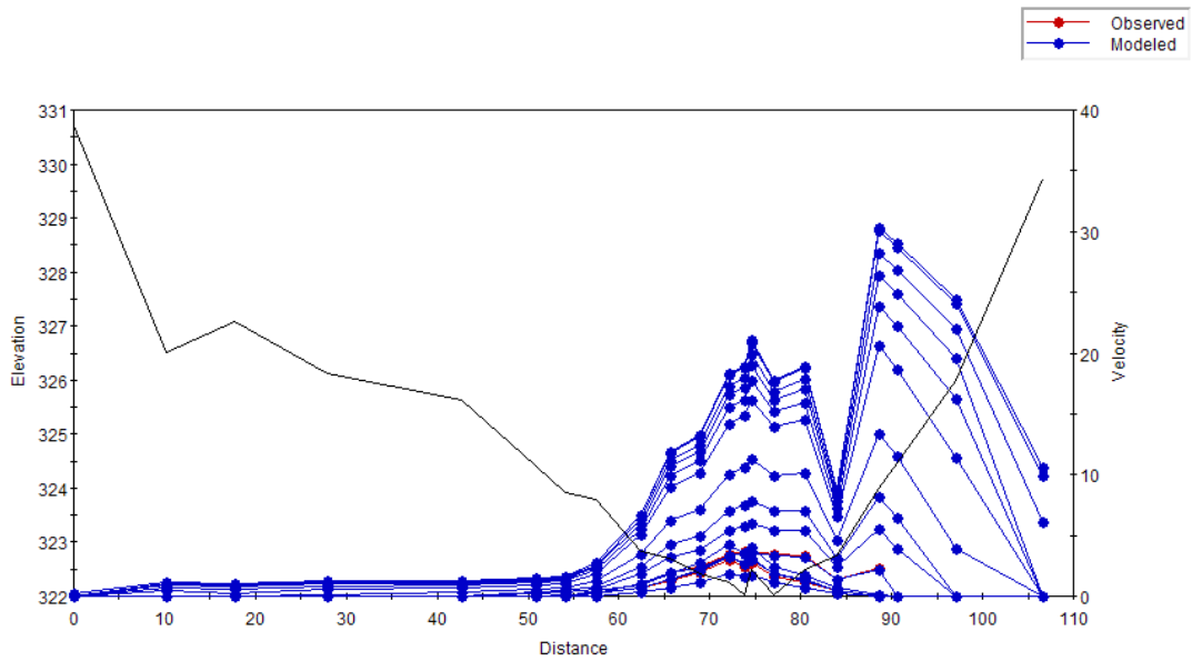
Figure C.28 Plot of the simulated velocity profiles for the Belly River – Study Reach 5 – Cross Section 6.
