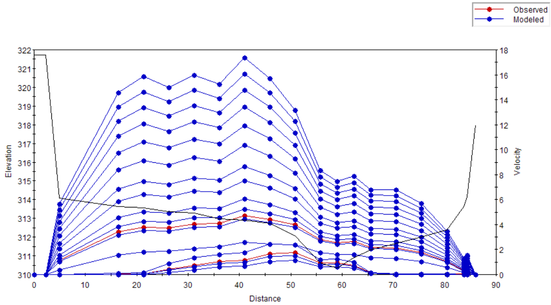
Figure C.13 Plot of the simulated velocity profiles for the Belly River – Study Reach 2 – Cross Section 6.
