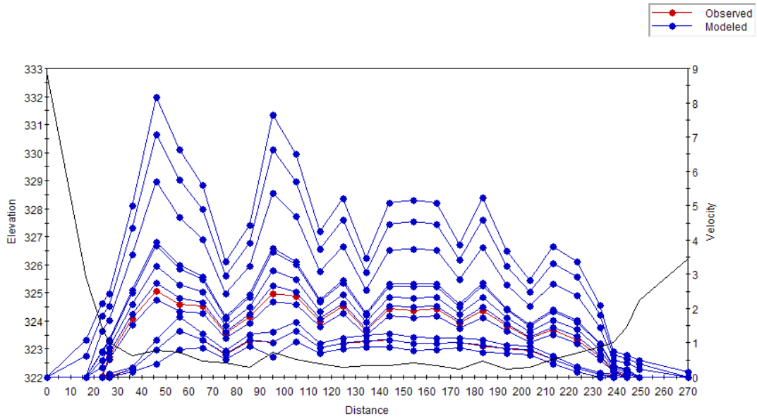
Figure C.7 Plot of the simulated velocity profiles for the Belly River – Study Reach 1 – Cross Section 7.
