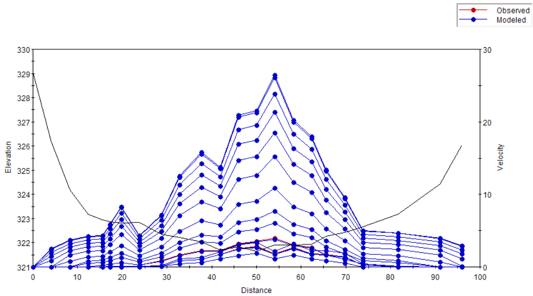
Figure C.25 Plot of the simulated velocity profiles for the Belly River – Study Reach 5 – Cross Section 3.
