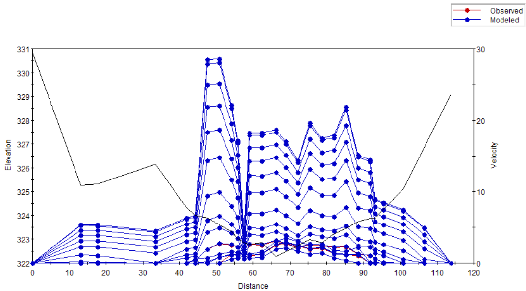
Figure C.26 Plot of the simulated velocity profiles for the Belly River – Study Reach 5 – Cross Section 4.
