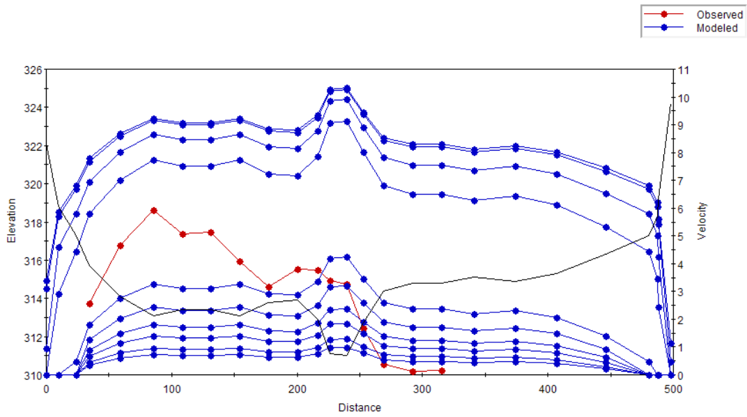
Figure C.33 Plot of the simulated velocity profiles for the Bow River – Study Reach 1 – Cross Section 3.
