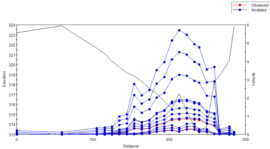
Figure C.1 Plot of the simulated velocity profiles for the Belly River – Study Reach 1 – Cross Section 1.
