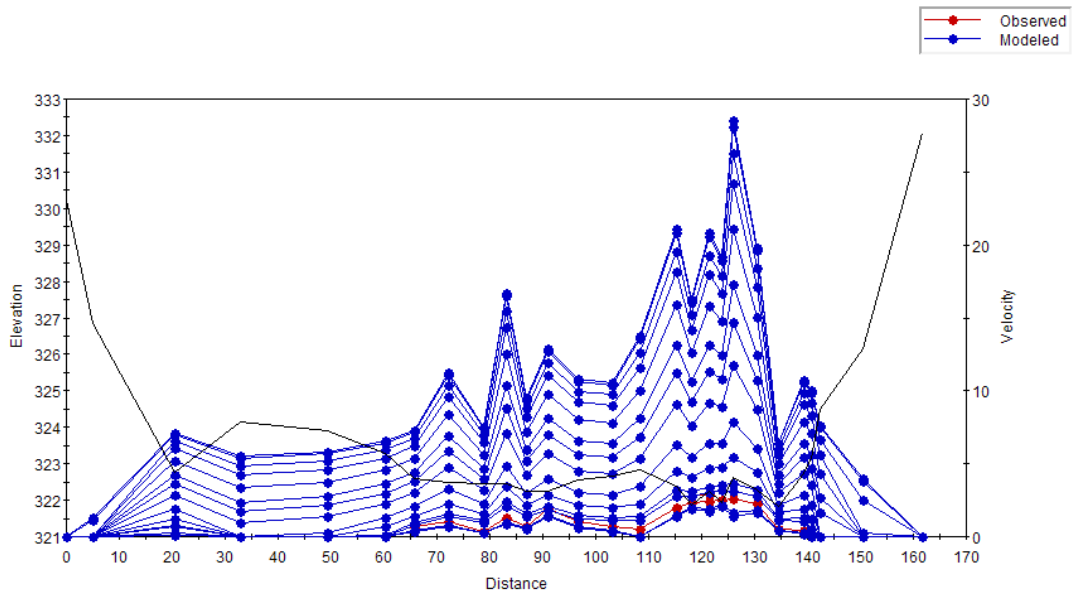
Figure C.22 Plot of the simulated velocity profiles for the Belly River – Study Reach 4 – Cross Section 7.
