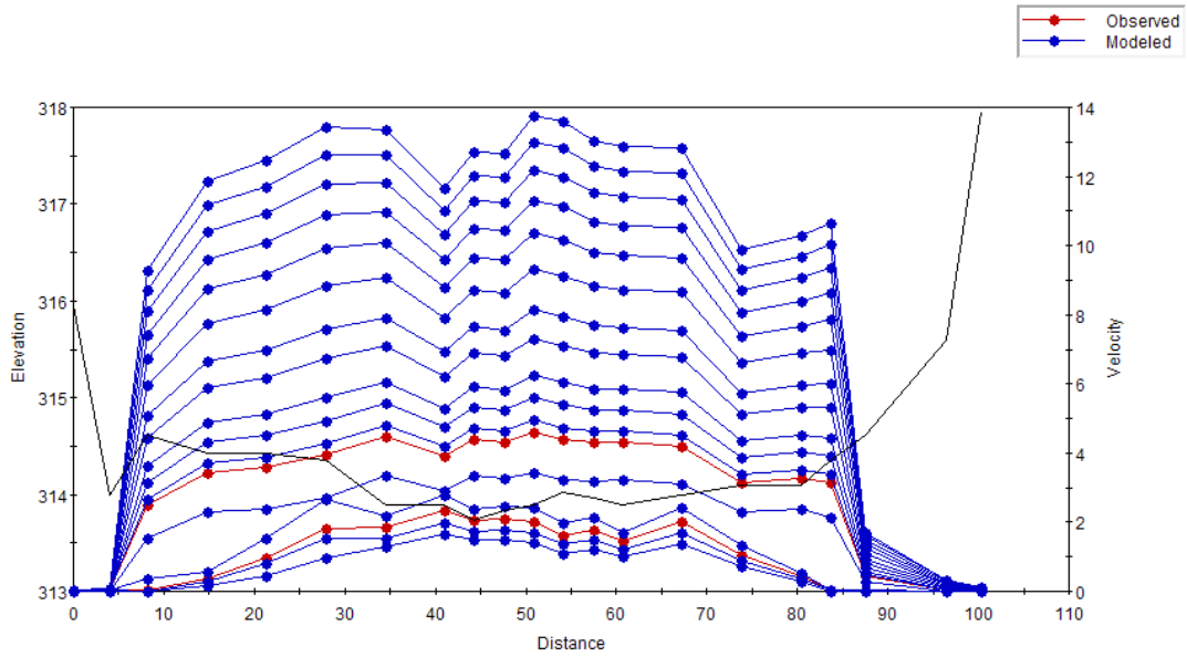
Figure C.15 Plot of the simulated velocity profiles for the Belly River – Study Reach 2 – Cross Section 8.
