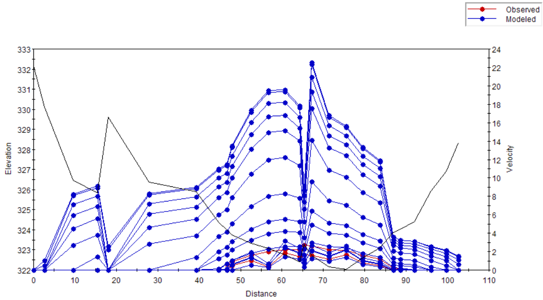
Figure C.27 Plot of the simulated velocity profiles for the Belly River – Study Reach 5 – Cross Section 5.
