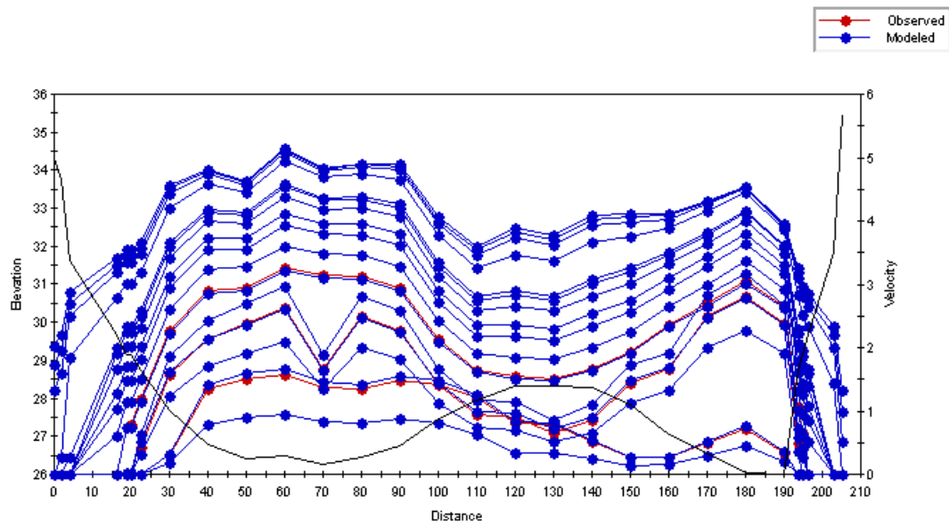
Figure C.101 Plot of the simulated velocity profiles for the Old Man River – Study Reach 5 – Cross Section 5.
