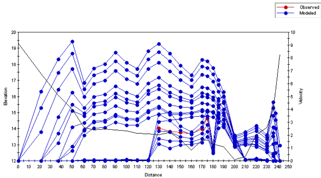
Figure C.93 Plot of the simulated velocity profiles for the Old Man River – Study Reach 4 – Cross Section 5.
