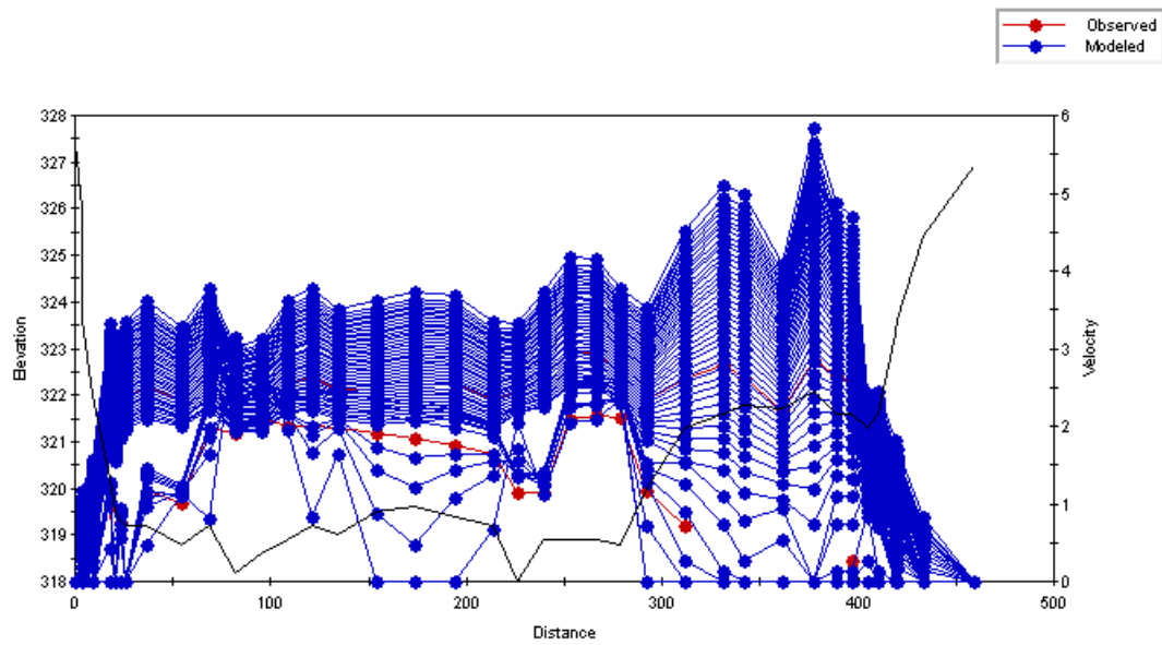
Figure C.110 Plot of the simulated velocity profiles for the Red Deer River – Study Reach 1 – Cross Section 2.
