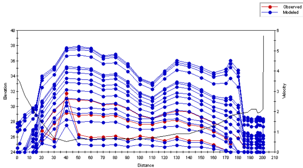
Figure C.100 Plot of the simulated velocity profiles for the Old Man River – Study Reach 5 – Cross Section 4.
