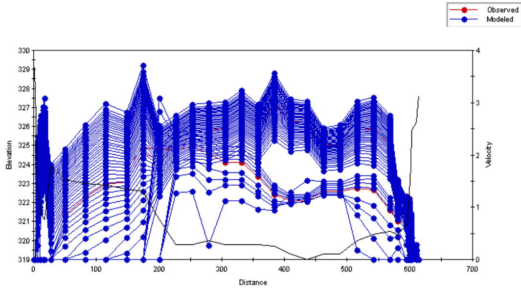
Figure C.111 Plot of the simulated velocity profiles for the Red Deer River – Study Reach 1 – Cross Section 3.
