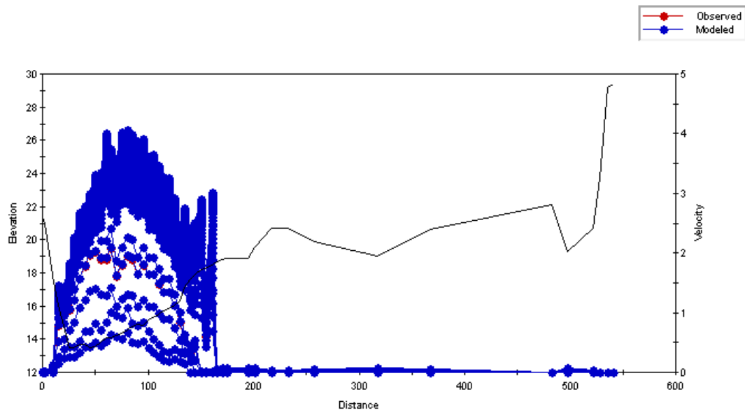
Figure C.106 Plot of the simulated velocity profiles for the Old Man River – Study Reach 6 – Cross Section 4.
