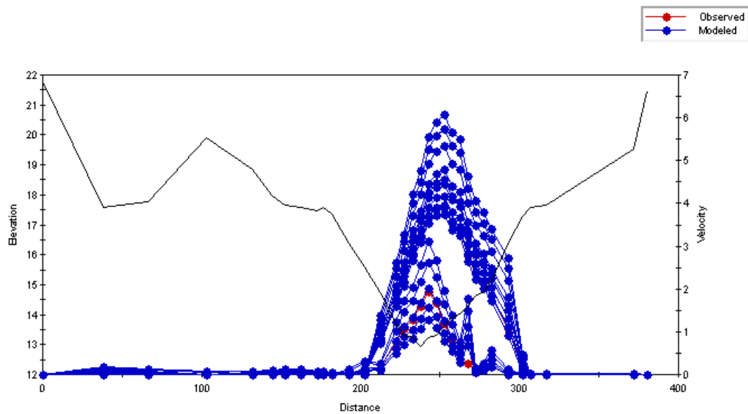
Figure C.96 Plot of the simulated velocity profiles for the Old Man River – Study Reach 4 – Cross Section 8.
