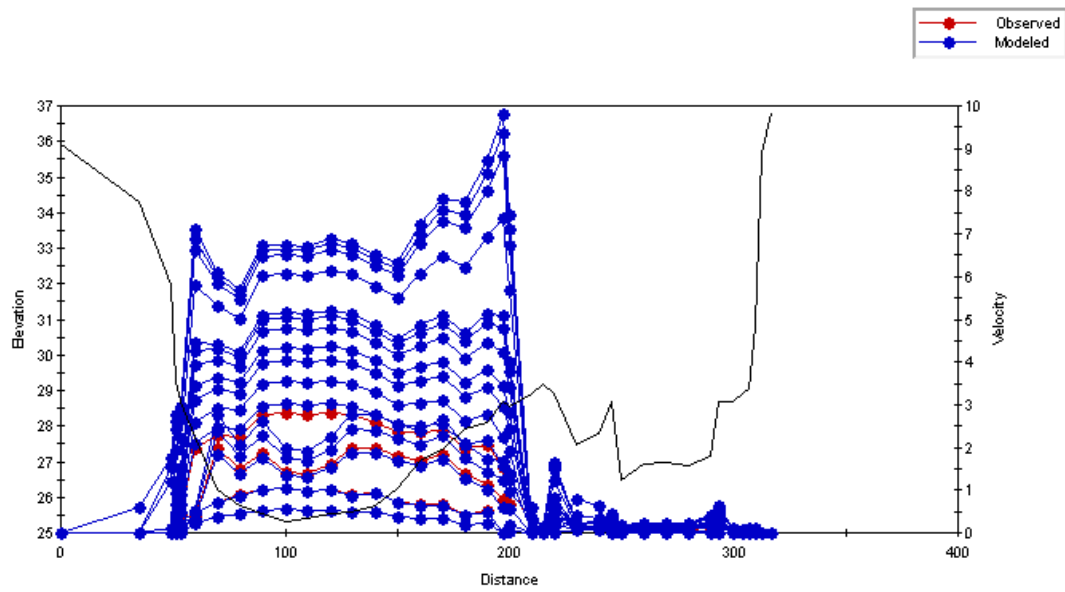
Figure C.99 Plot of the simulated velocity profiles for the Old Man River – Study Reach 5 – Cross Section 3.
