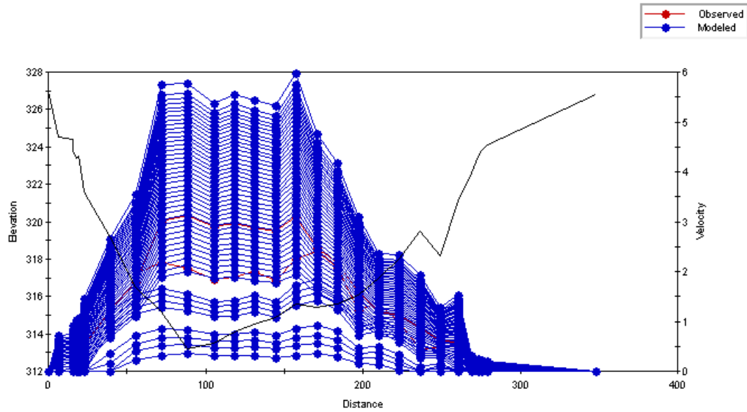
Figure C.109 Plot of the simulated velocity profiles for the Red Deer River – Study Reach 1 – Cross Section 1.
