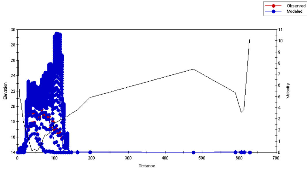
Figure C.107 Plot of the simulated velocity profiles for the Old Man River – Study Reach 6 – Cross Section 5.
