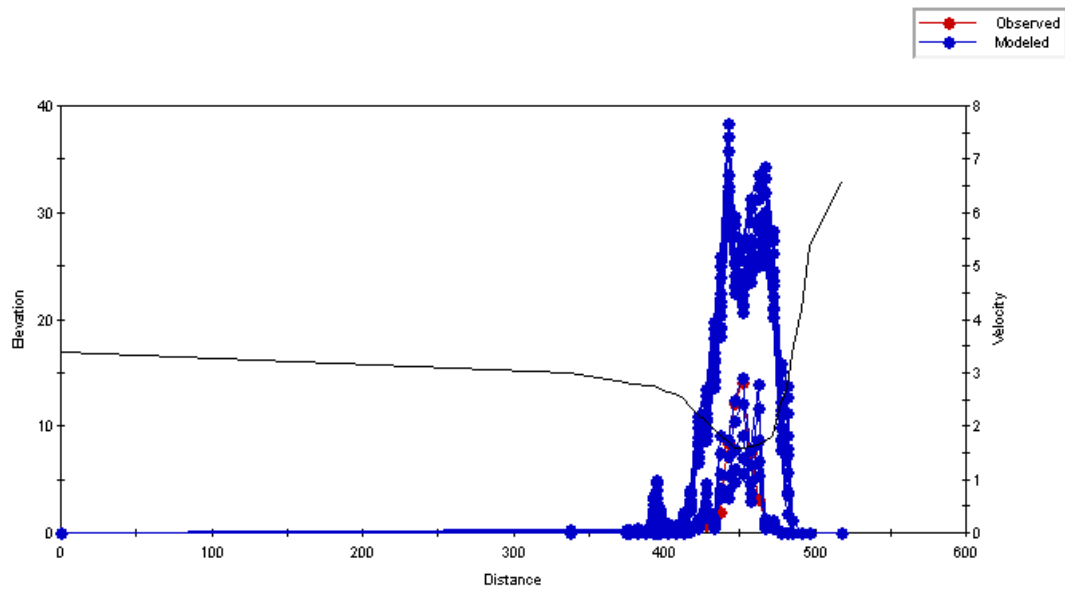
Figure C.89 Plot of the simulated velocity profiles for the Old Man River – Study Reach 4 – Cross Section 1.
