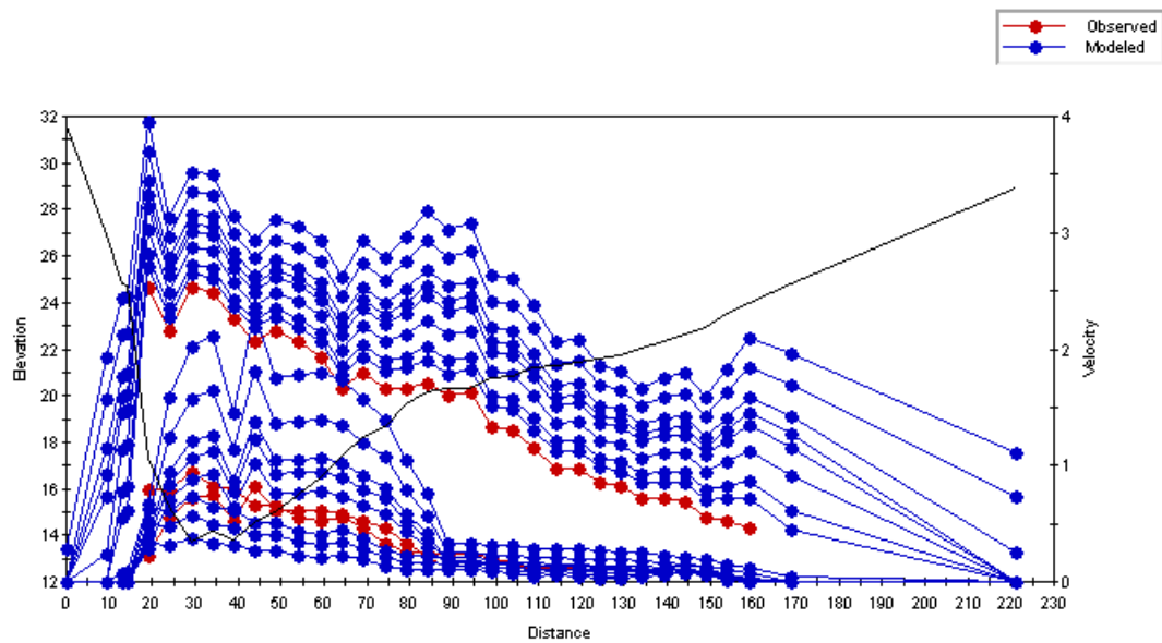
Figure C.80 Plot of the simulated velocity profiles for the Old Man River – Study Reach 2 – Cross Section 4.
