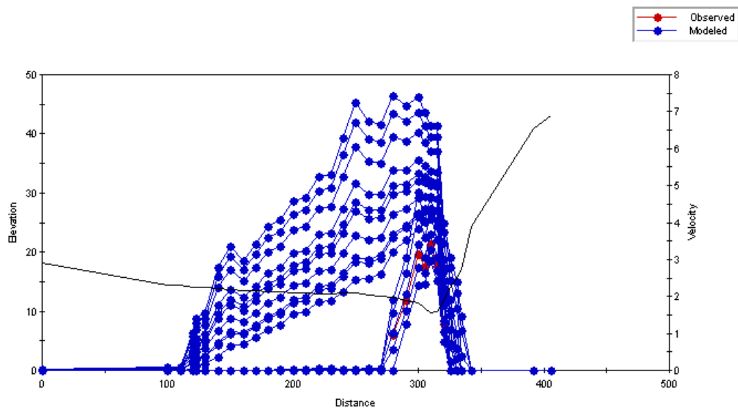
Figure C.90 Plot of the simulated velocity profiles for the Old Man River – Study Reach 4 – Cross Section 2.
