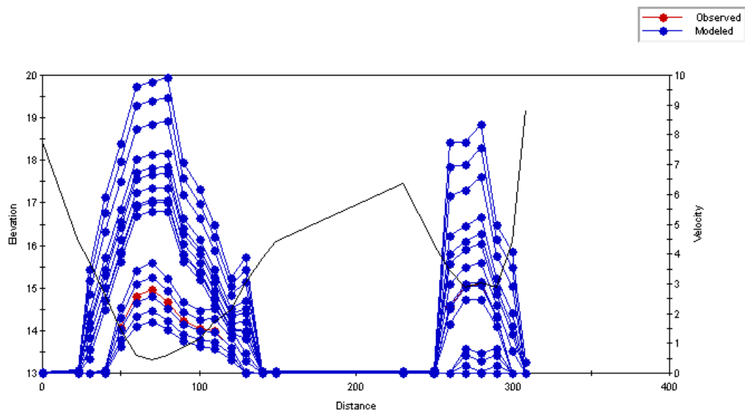
Figure C.94 Plot of the simulated velocity profiles for the Old Man River – Study Reach 4 – Cross Section 6.
