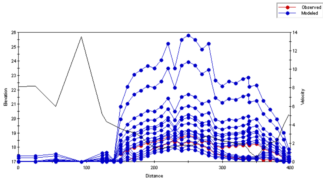
Figure C.87 Plot of the simulated velocity profiles for the Old Man River – Study Reach 3 – Cross Section 4.
