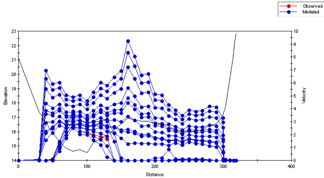
Figure C.95 Plot of the simulated velocity profiles for the Old Man River – Study Reach 4 – Cross Section 7.
