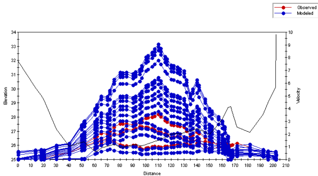
Figure C.102 Plot of the simulated velocity profiles for the Old Man River – Study Reach 5 – Cross Section 6.
