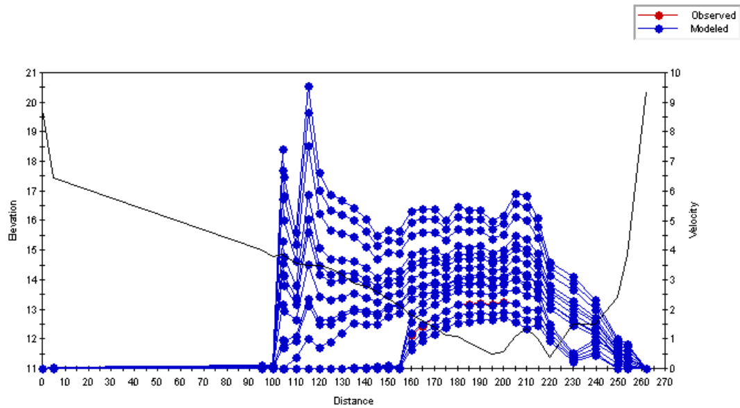
Figure C.92 Plot of the simulated velocity profiles for the Old Man River – Study Reach 4 – Cross Section 4.
