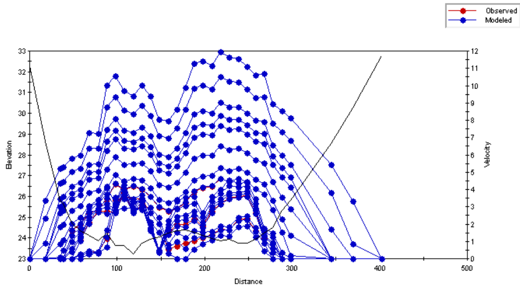
Figure C.83 Plot of the simulated velocity profiles for the Old Man River – Study Reach 2 – Cross Section 7.
