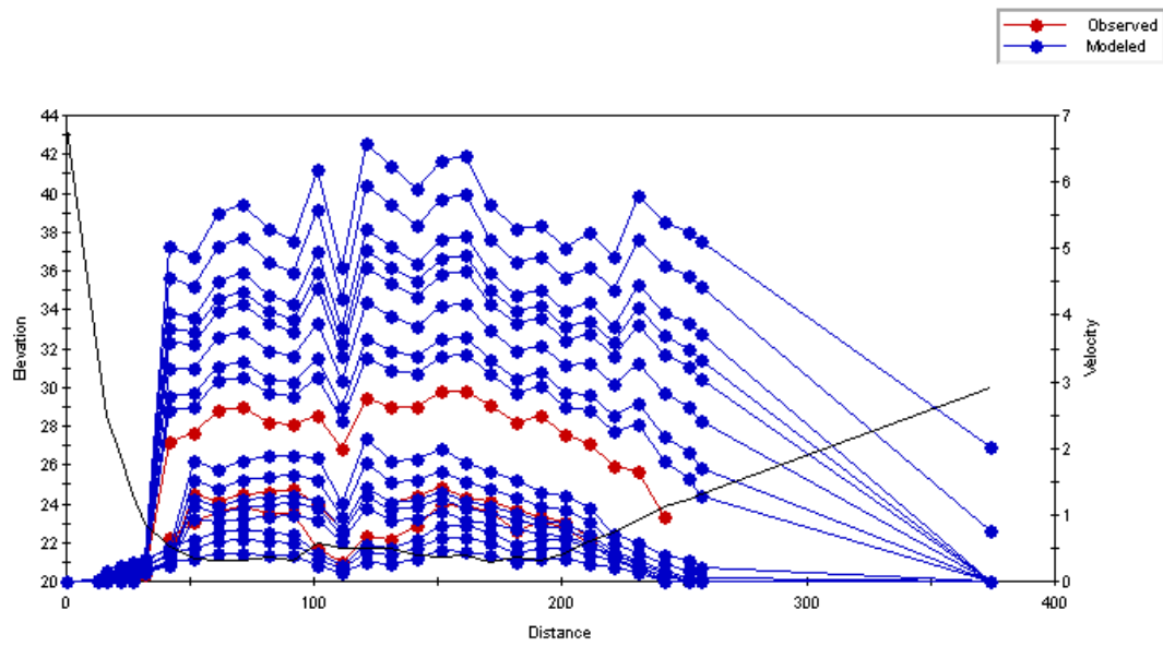
Figure C.79 Plot of the simulated velocity profiles for the Old Man River – Study Reach 2 – Cross Section 3.
