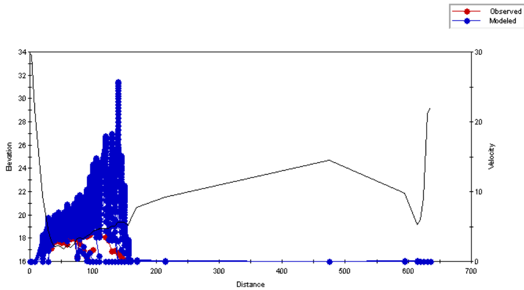
Figure C.108 Plot of the simulated velocity profiles for the Old Man River – Study Reach 6 – Cross Section 6.
