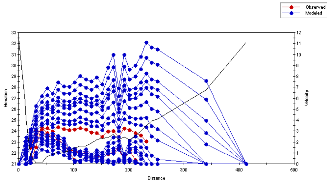
Figure C.81 Plot of the simulated velocity profiles for the Old Man River – Study Reach 2 – Cross Section 5.
