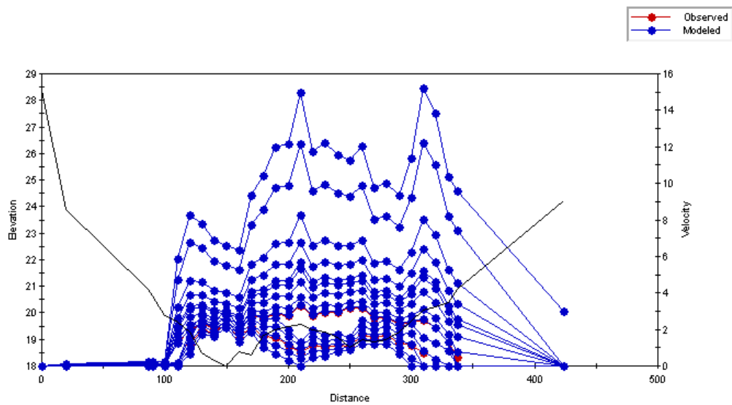
Figure C.88 Plot of the simulated velocity profiles for the Old Man River – Study Reach 3 – Cross Section 5.
