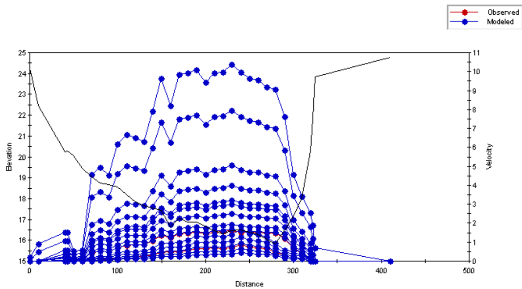
Figure C.86 Plot of the simulated velocity profiles for the Old Man River – Study Reach 3 – Cross Section 3.
