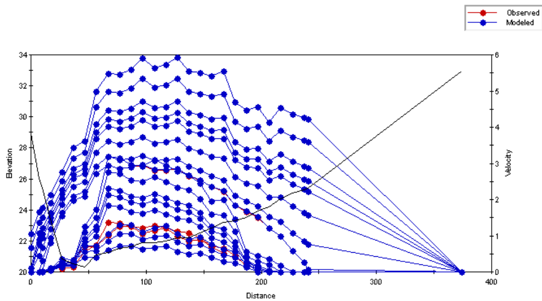
Figure C.82 Plot of the simulated velocity profiles for the Old Man River – Study Reach 2 – Cross Section 6.
