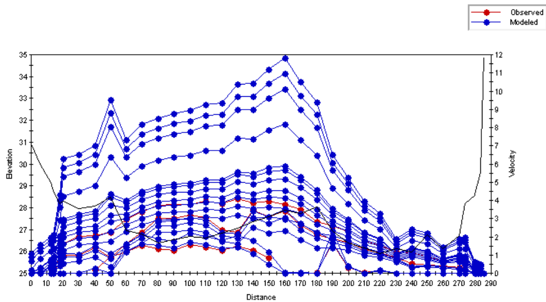
Figure C.98 Plot of the simulated velocity profiles for the Old Man River – Study Reach 5 – Cross Section 2.
