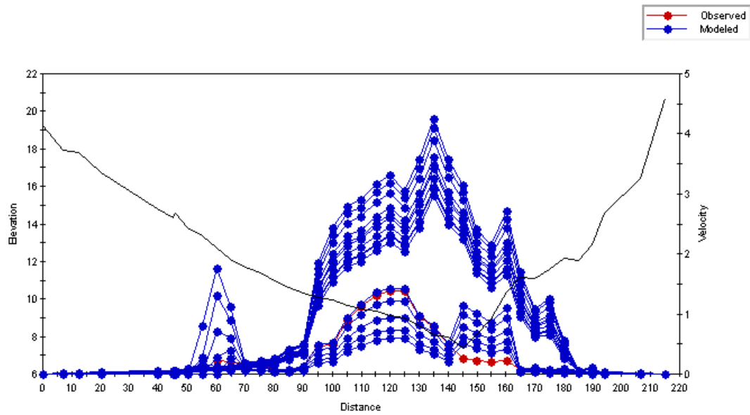
Figure C.91 Plot of the simulated velocity profiles for the Old Man River – Study Reach 4 – Cross Section 3.
