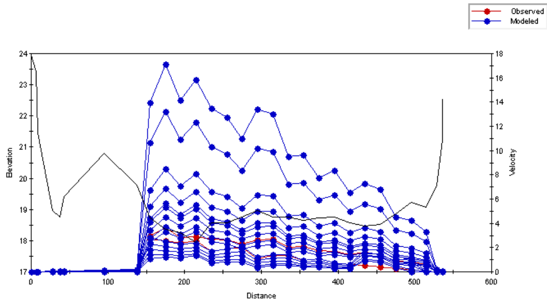
Figure C.84 Plot of the simulated velocity profiles for the Old Man River – Study Reach 3 – Cross Section 1.
