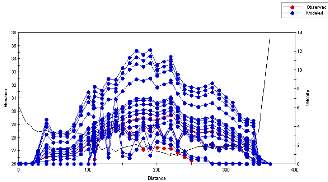
Figure C.97 Plot of the simulated velocity profiles for the Old Man River – Study Reach 5 – Cross Section 1.
