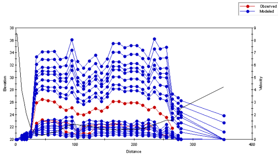
Figure C.78 Plot of the simulated velocity profiles for the Old Man River – Study Reach 2 – Cross Section 2.
