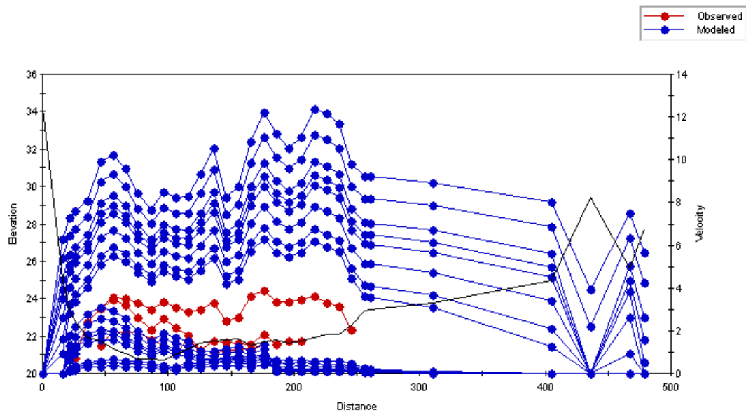
Figure C.77 Plot of the simulated velocity profiles for the Old Man River – Study Reach 2 – Cross Section 1.
