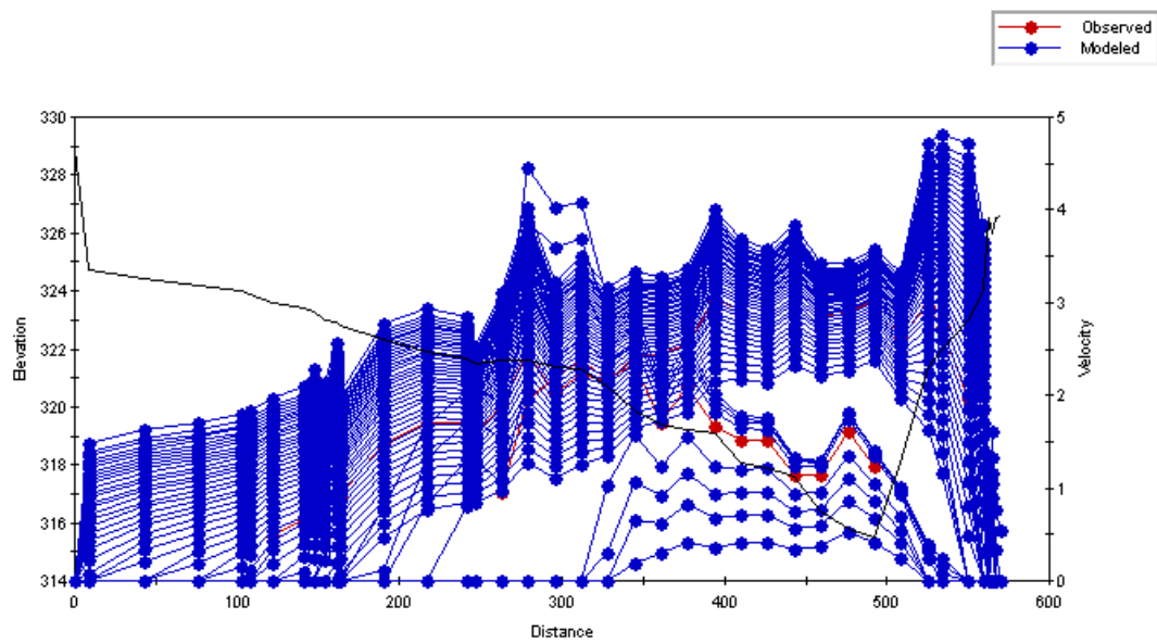
Figure C.112 Plot of the simulated velocity profiles for the Red Deer River – Study Reach 1 – Cross Section 4.
