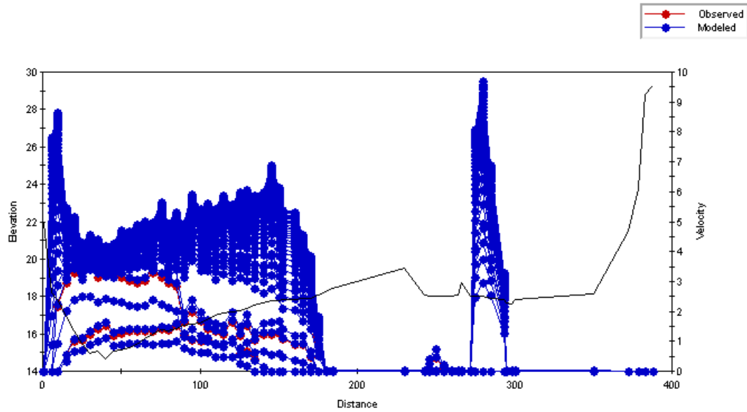
Figure C.105 Plot of the simulated velocity profiles for the Old Man River – Study Reach 6 – Cross Section 3.
