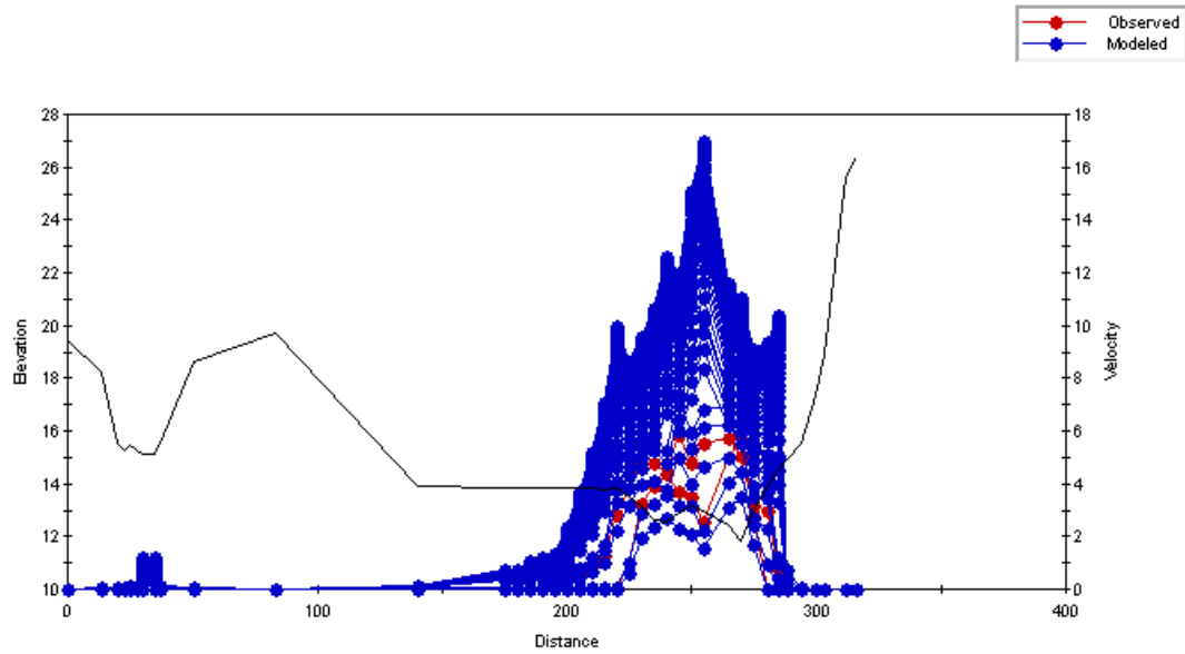
Figure C.103 Plot of the simulated velocity profiles for the Old Man River – Study Reach 6 – Cross Section 1.
