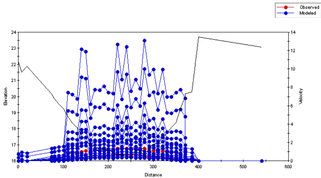
Figure C.85 Plot of the simulated velocity profiles for the Old Man River – Study Reach 3 – Cross Section 2.
