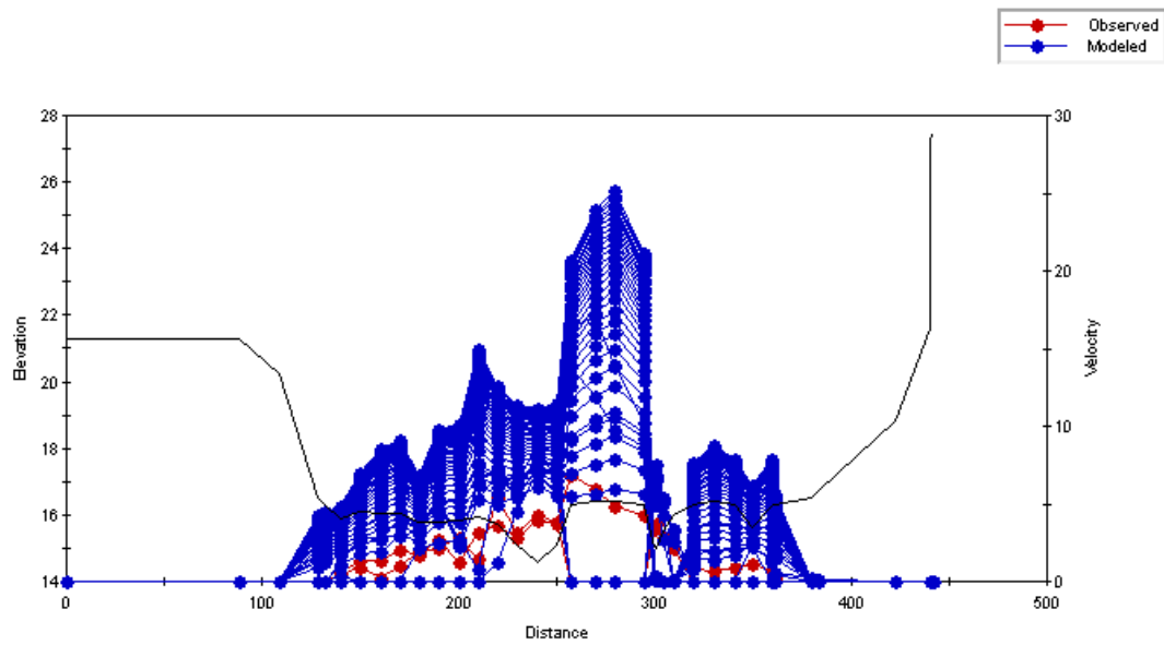
Figure C.104 Plot of the simulated velocity profiles for the Old Man River – Study Reach 6 – Cross Section 2.
