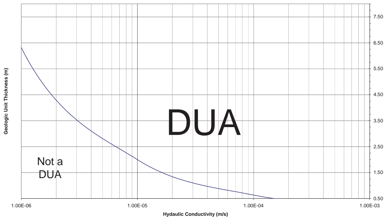
Figure 2. Minimum thickness required to meet DUA condition for an unconfined aquifer. Site-specific calculations can be made using the method in Section E.4
