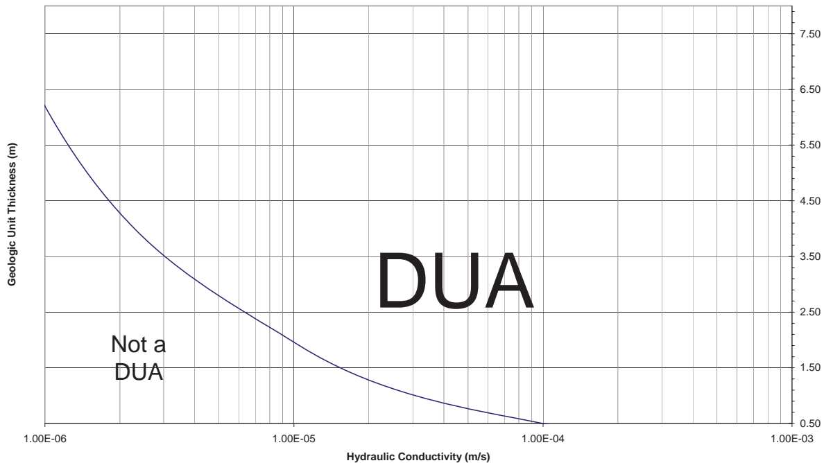
Figure 1. Minimum thickness required to meet DUA condition for a confined aquifer. Site-specific calculations can be made using the method in Section E.4
