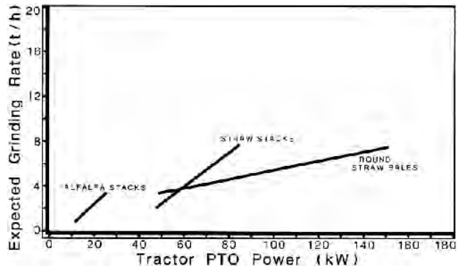
FIGURE 8. Determining Expected Average Grinding Rates With the Bearcat 4200 for Various Tractor Sizes when Using a 51 mm (2 in) Screen.
