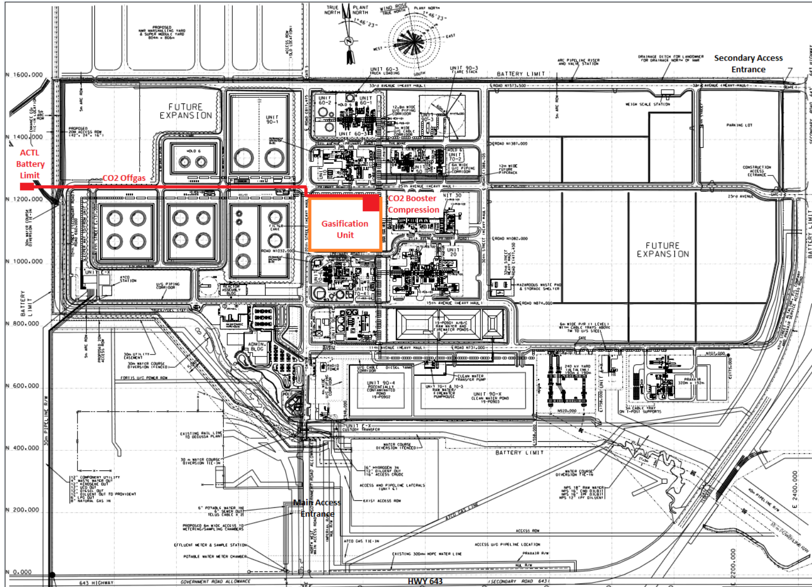
Figure 1.9.1 – NWR Sturgeon Refinery Plot Plan
