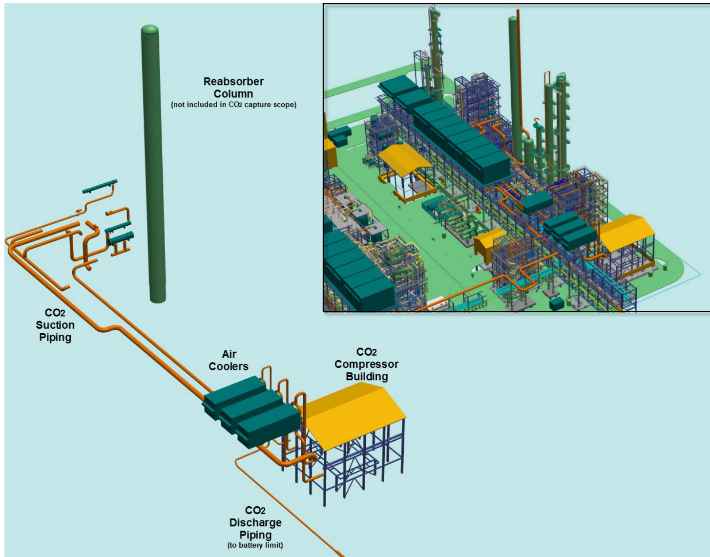
Figure 1.9.6 –3D NW View of CO 2 Piping Layout
