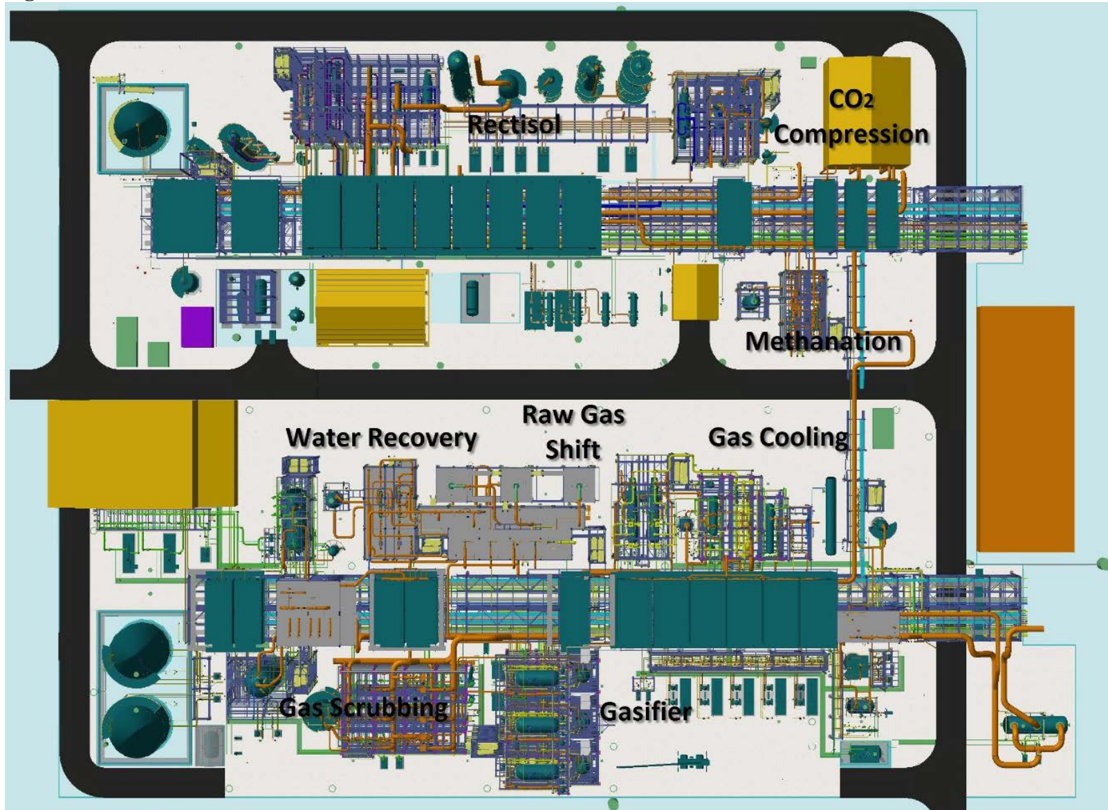
Figure 1.9.3 – Gasifier Unit 3D Plan View
