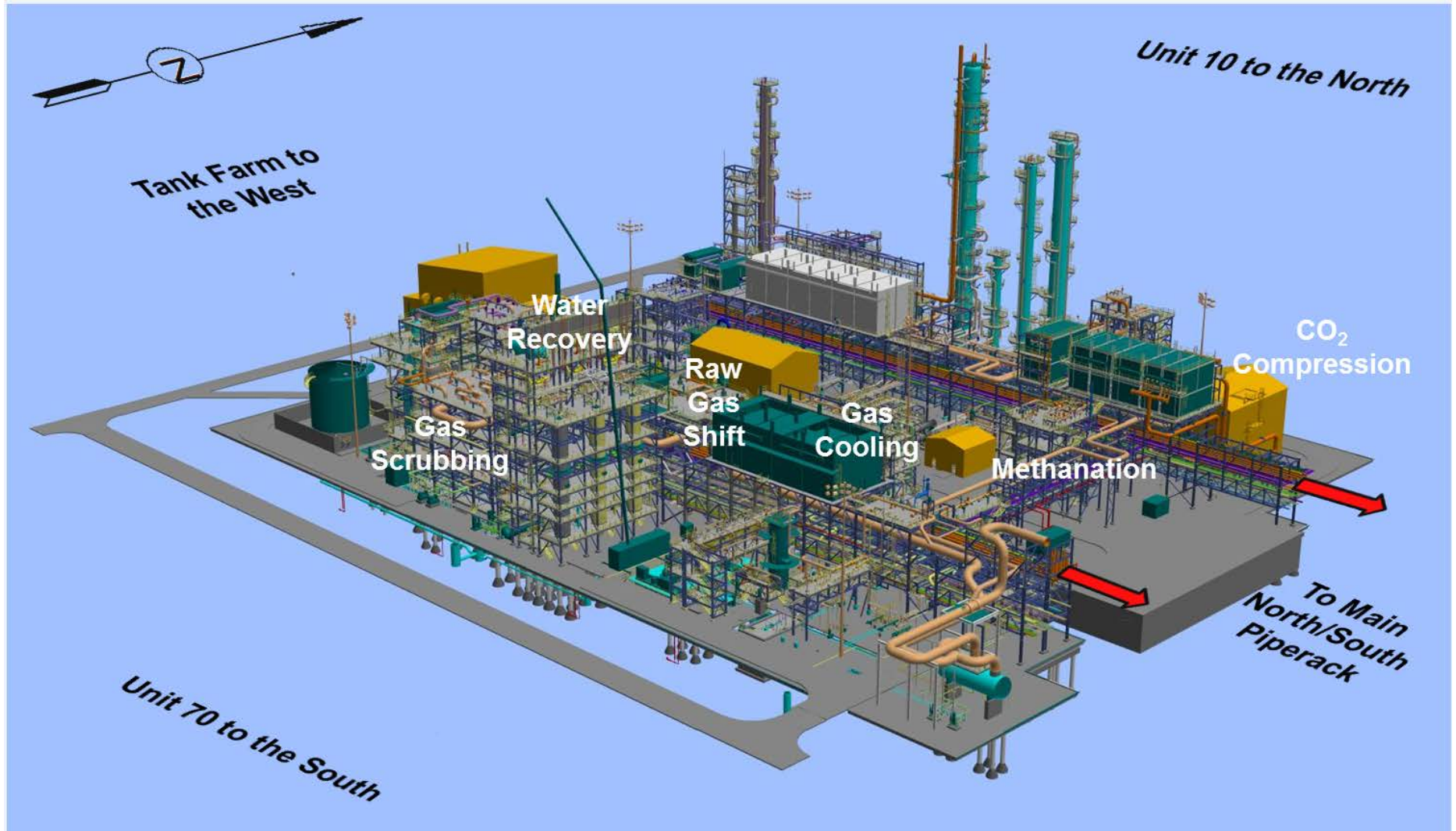
Figure 1.9.4 – Gasifier Unit – 3D NW View
