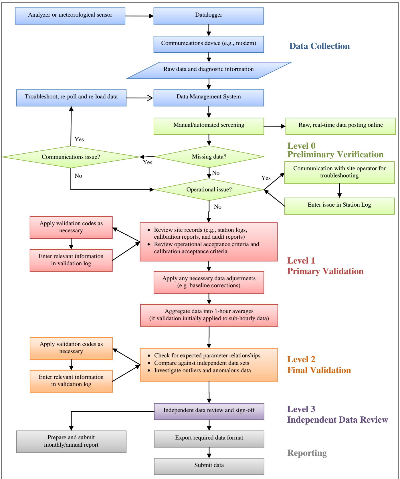
Figure 1 Data Collection and Management Process Flow Chart
