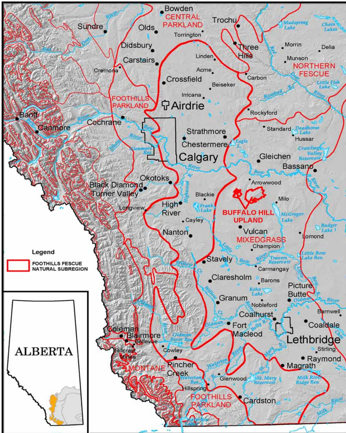
Figure 3: Foothills Fescue Natural Subregion with Hillshade Model (Digital Elevation Model)
