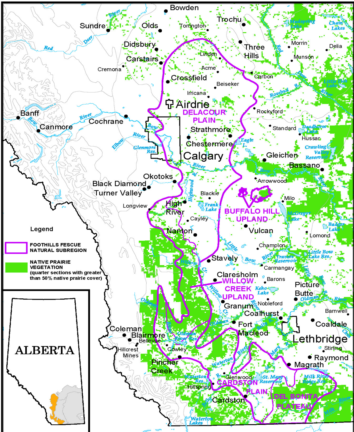
Figure 2: Ecodistricts in the Foothills Fescue Natural Subregion, and the Buffalo Hill Upland
