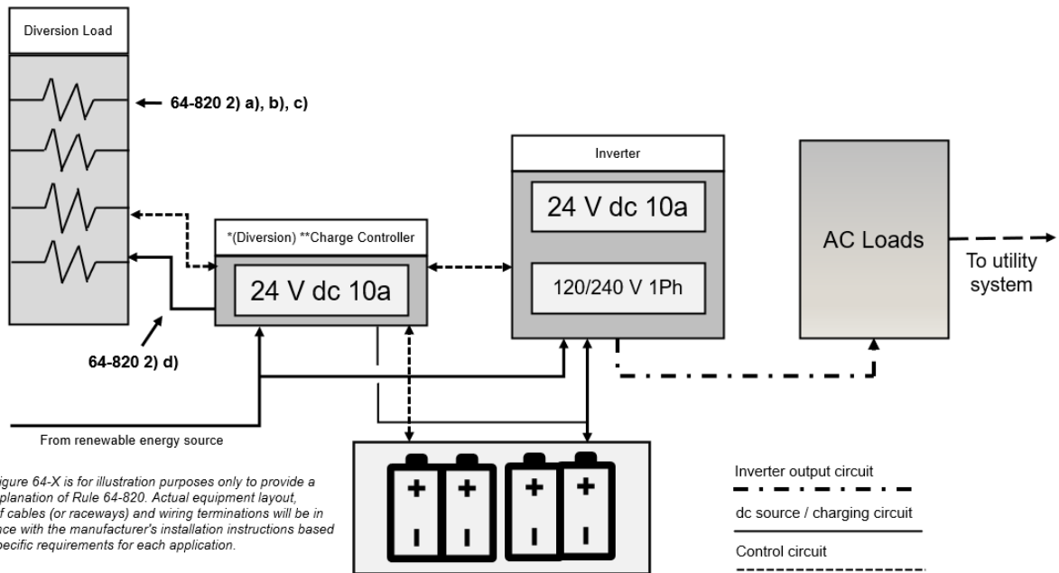
Figure B64-XX Diversion Charge Control System
