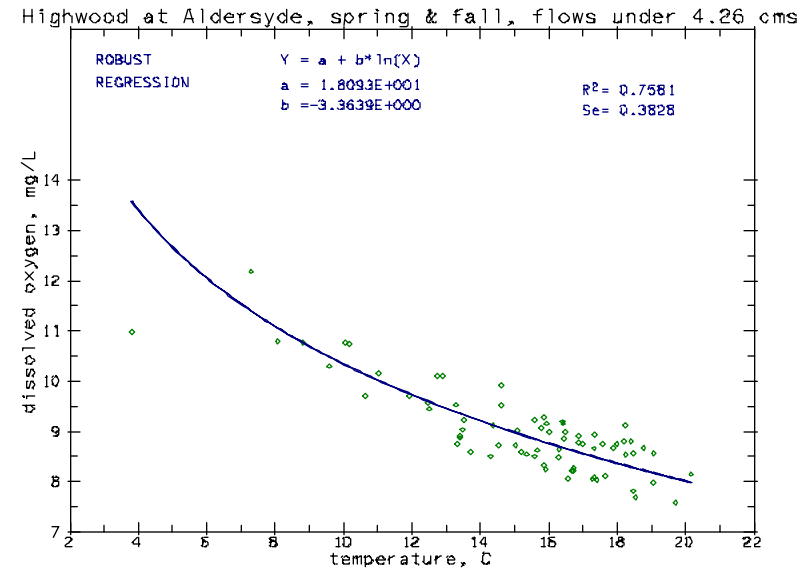
Figure 11 Regression between daily minimum dissolved oxygen and maximum water temperature in the lower Highwood River at flows <4.26 \text{ m}^3/\text{s} in spring and fall, 1990-97
