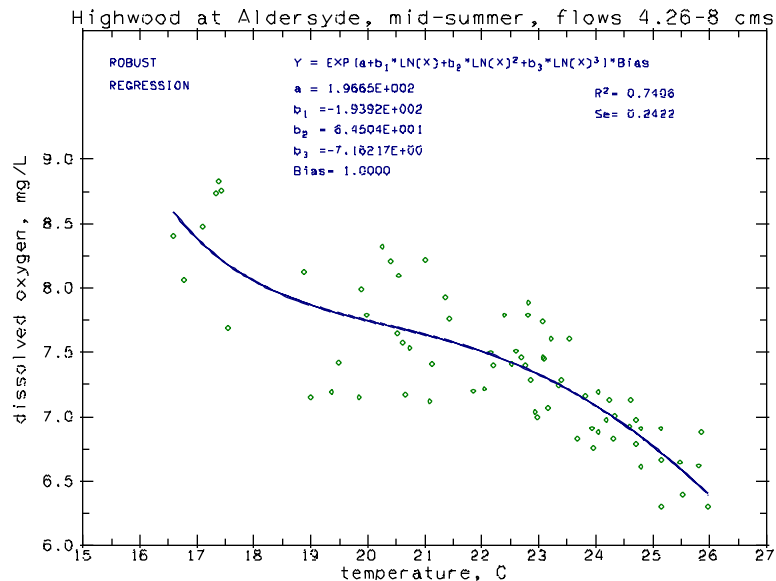
Figure 6 Regression between daily minimum dissolved oxygen and maximum water temperature in the lower Highwood River at flows 4.26\text{--}8 \text{ m}^3/\text{s} in midsummer, 1990-97
