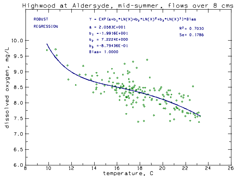
Figure 4 Regression between daily minimum dissolved oxygen and maximum water temperature in the lower Highwood River in midsummer, 1990-97
