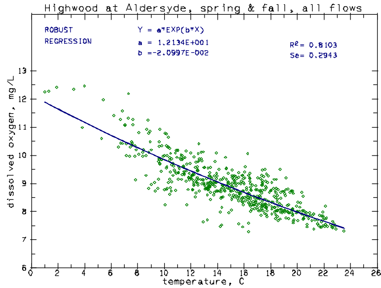
Figure 8 Regression between daily minimum dissolved oxygen and maximum water temperature in the lower Highwood River in spring and fall, 1990-97
