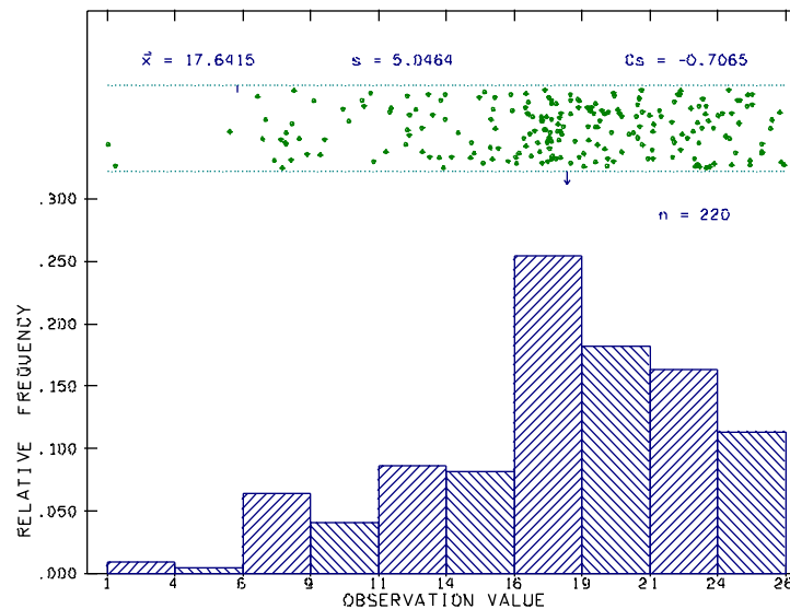
Figure 2 Maximum daily water temperature in the Highwood River at Aldersyde at flows of 4.26\text{--}8 \text{ m}^3/\text{s} , 1990-97
