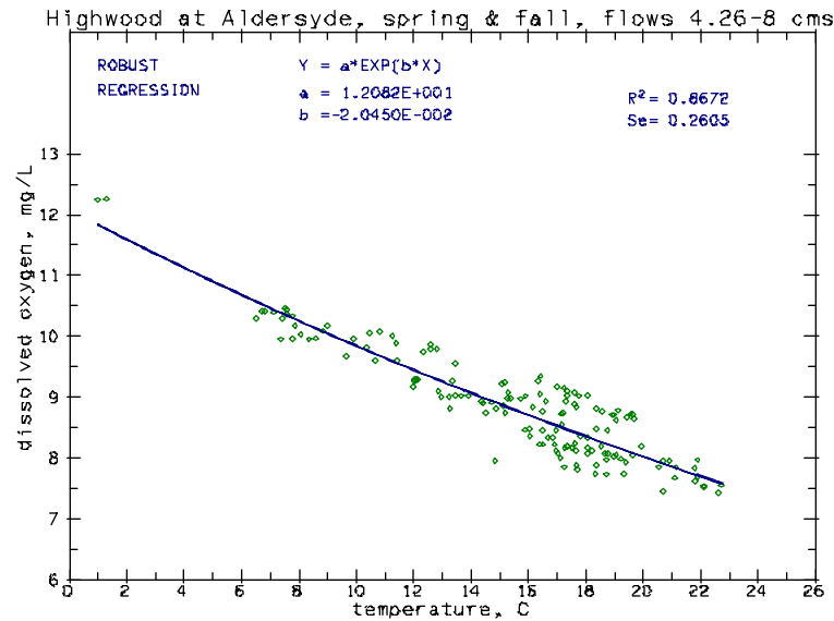
Figure 10 Regression between daily minimum dissolved oxygen and maximum water temperature in the lower Highwood River at flows 4.26\text{--}8 \text{ m}^3/\text{s} in spring and fall, 1990-97
