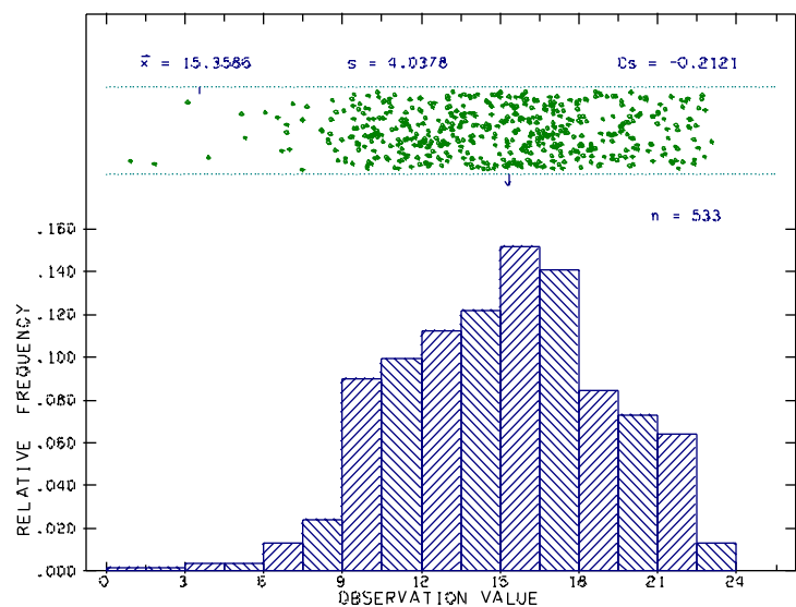
Figure 1 Maximum daily water temperature in the Highwood River at Aldersyde at flows > 8 \text{ m}^3/\text{s} , 1990-97
