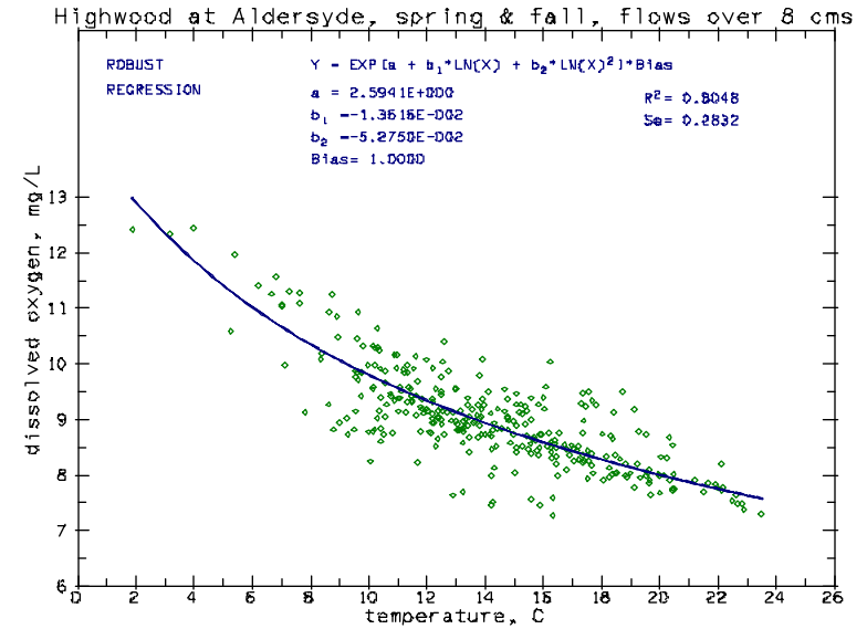
Figure 9 Regression between daily minimum dissolved oxygen and maximum water temperature in the lower Highwood River at flows >8 \text{ m}^3/\text{s} in spring and fall, 1990-97
