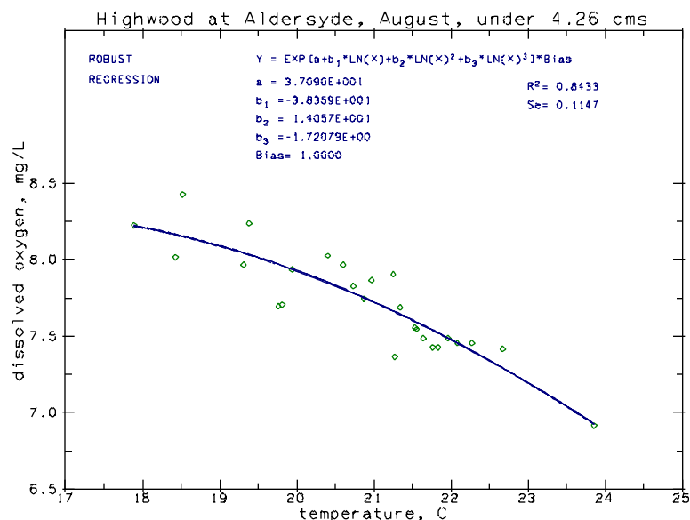
Figure 7 Regression between daily minimum dissolved oxygen and maximum water temperature in the lower Highwood River at flows < 4.26 \text{ m}^3/\text{s} in midsummer, 1990-97
