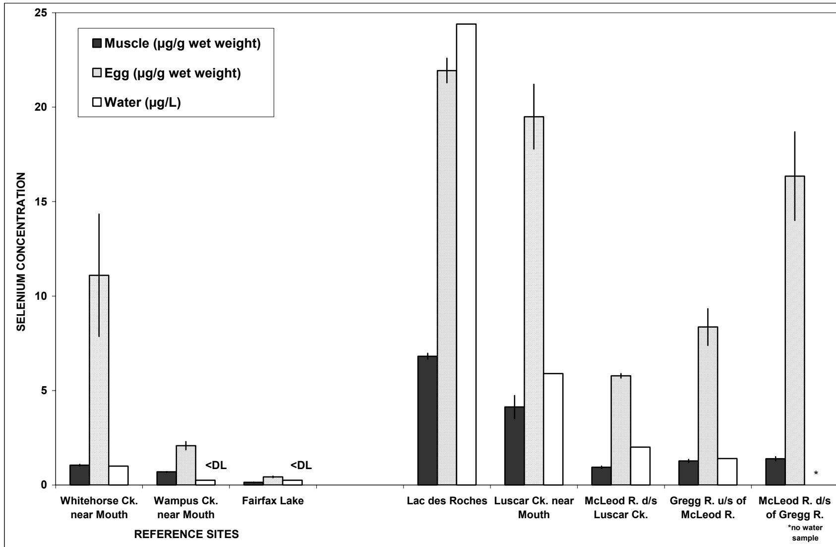
Figure 3. Concentrations of selenium in rainbow trout muscle and egg tissues (mean \pm standard error), and in water in spring 1999. Selenium concentrations were less than the detection level (DL = 0.5 \mu\text{g/L} ) in Wampus Creek and Fairfax Lake.
