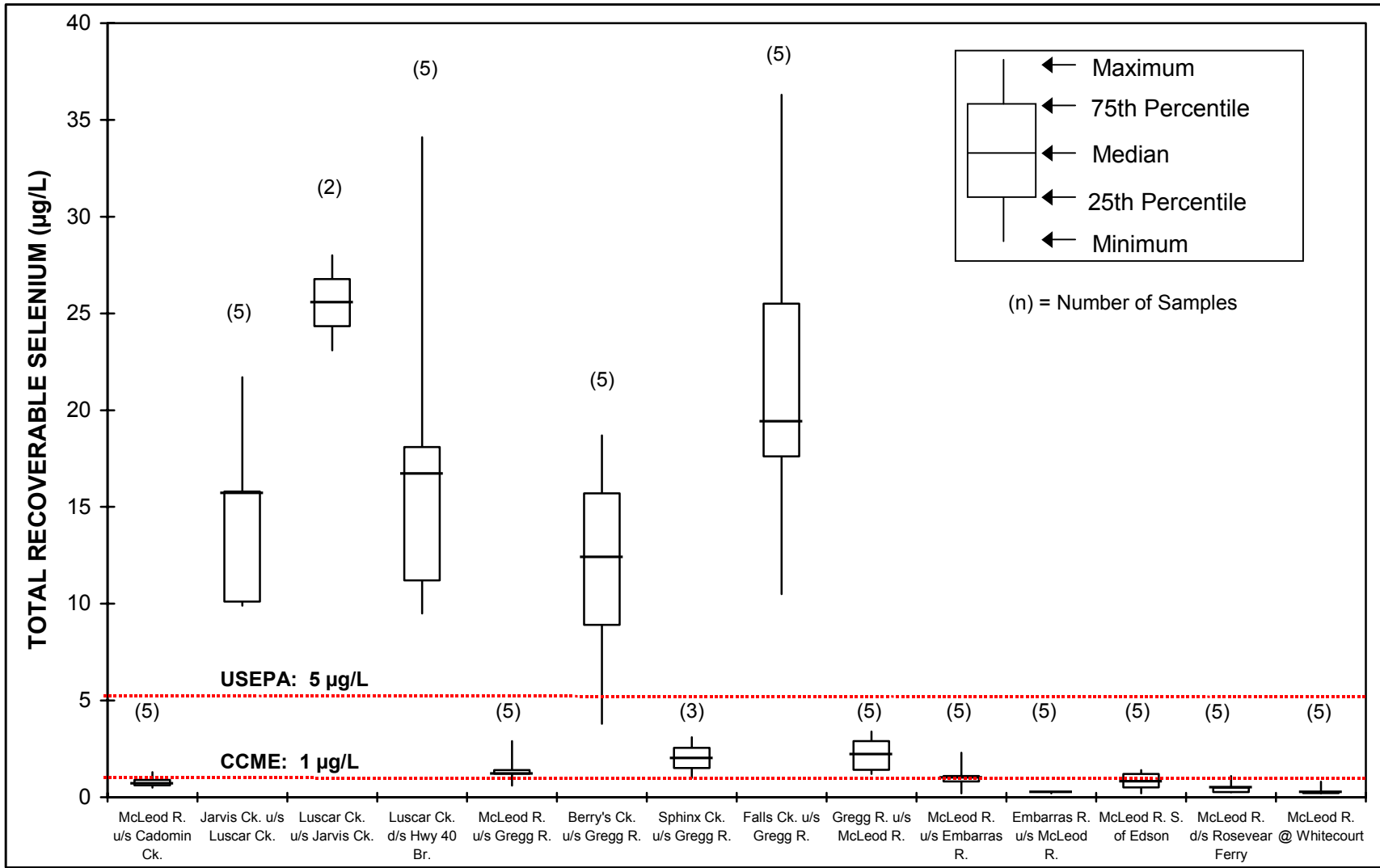
Figure 6. Box and whisker graphs showing the concentrations of selenium at sites sampled in the McLeod River Water Quality Study from September 1998 to September 1999.
