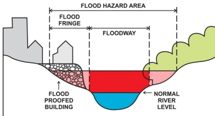
Cross-Section of Flood Hazard Area
