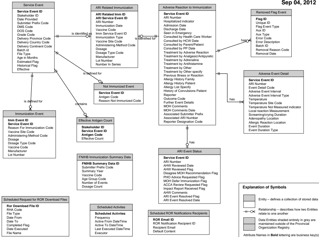
ImmARI Event Registry – Logical Data Model
