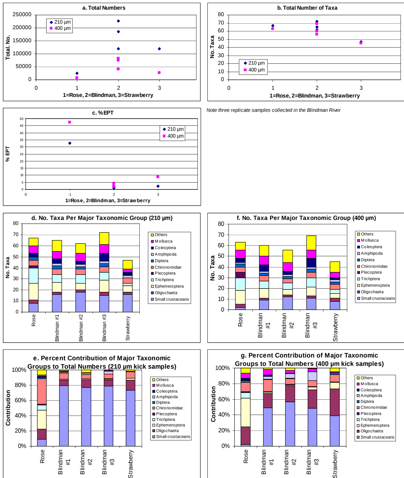
Figure 2 Benthic invertebrate data for three agricultural streams
