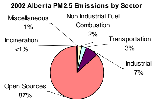
Figure A2 CAC emissions for CO, total PM, PM 10 and PM 2.5 in Alberta (data provided by Environment Canada).
