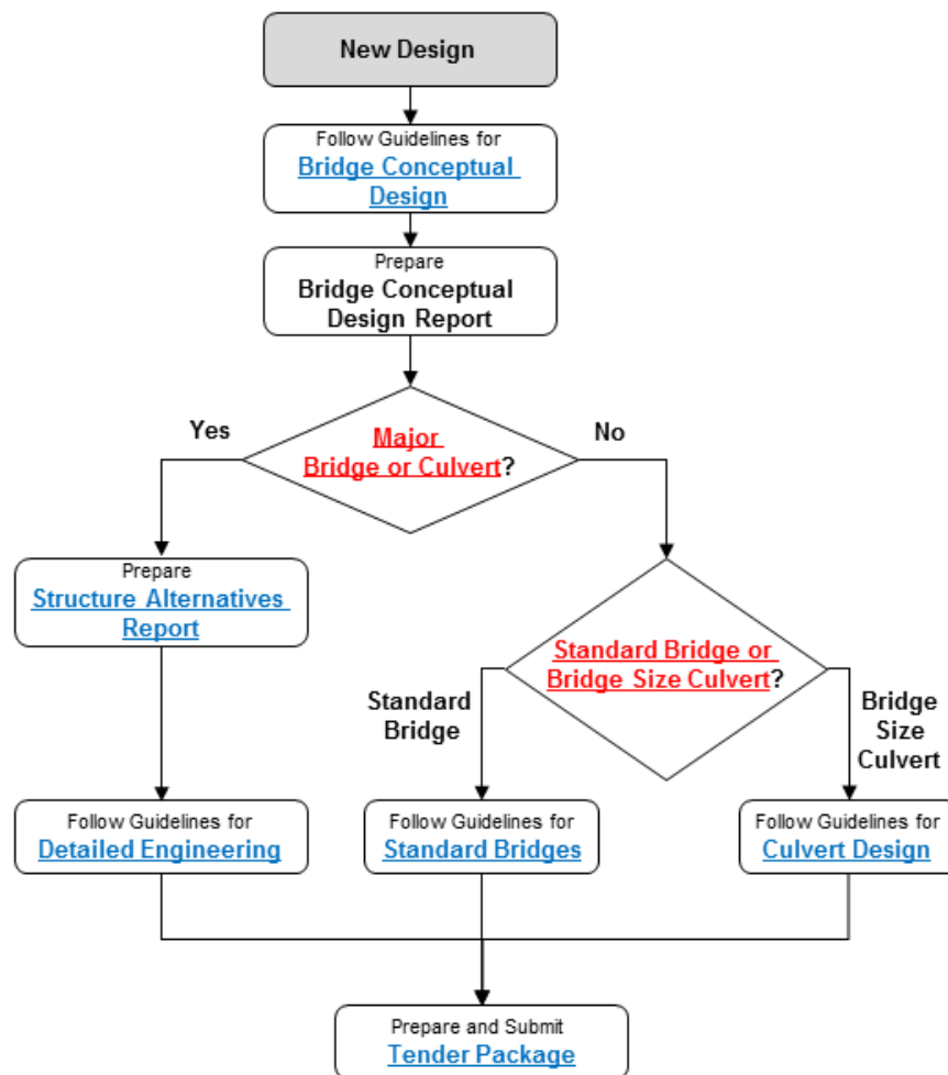
Figure 1: Bridge New Design Flowchart
