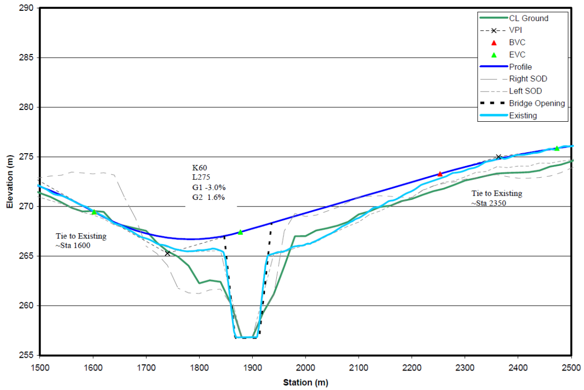
Figure 8: Potential Gradeline for Existing Alignment Downstream (Recommended)
