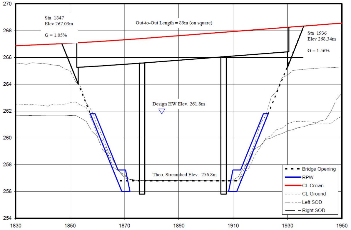
Figure 12: Recommended Alignment – Bridge Elevation View
