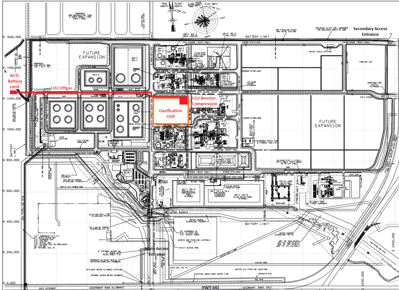
Figure 3 – North West Sturgeon Refinery Plot Plan
