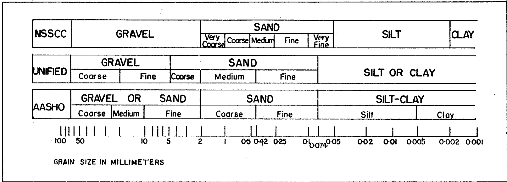
Figure 4. Comparison of particle size for the NSSCC, Unified and AASHO systems of textural classification. (Modified after Michalyna, Smith and Hopkins. 1968.)
