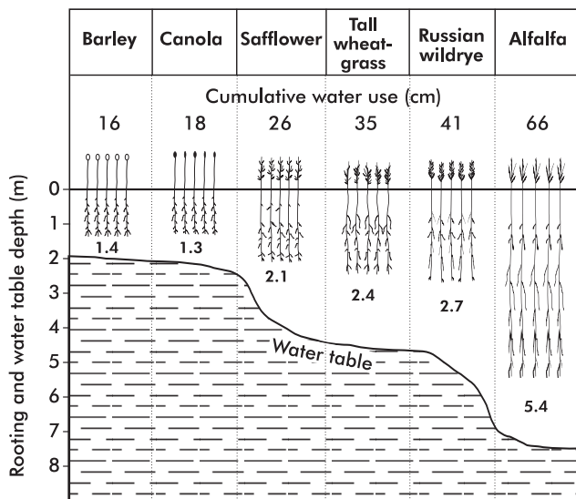
Figure 1 Cumulative water use and rooting depth of crops over a four-year period
