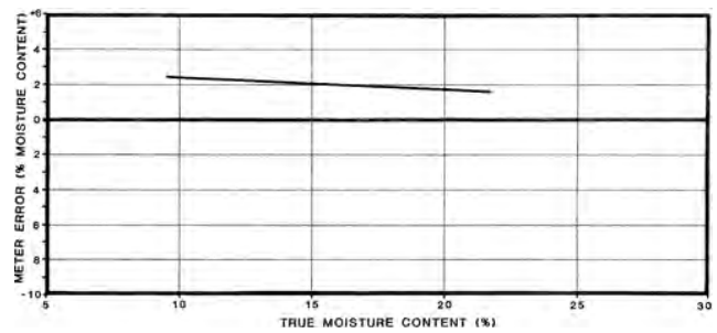
Figure 2. Deviations of Meter Readings for Qwik-Test in Wheat.
