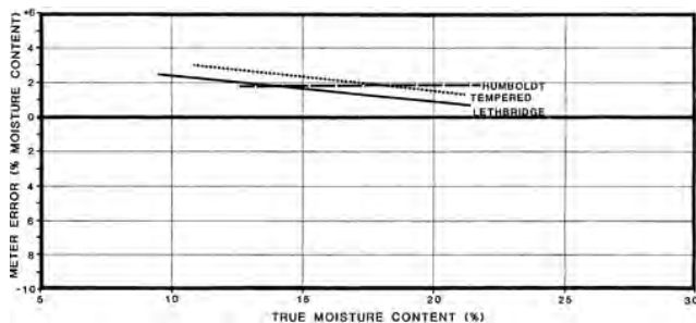
Figure 6. Deviations of Meter Readings for Qwik-Test in Three Different Types of Spring Wheat.
