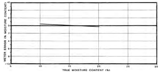
Figure 3. Deviations of Meter Readings for Qwik-Test in Barley.
