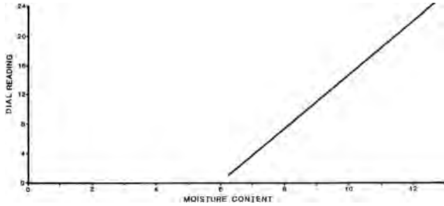
Figure 5. Calibration Curve for Qwik-Test in Rapeseed.
