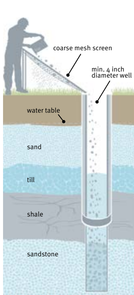
Figure 1: Plugging an old well
